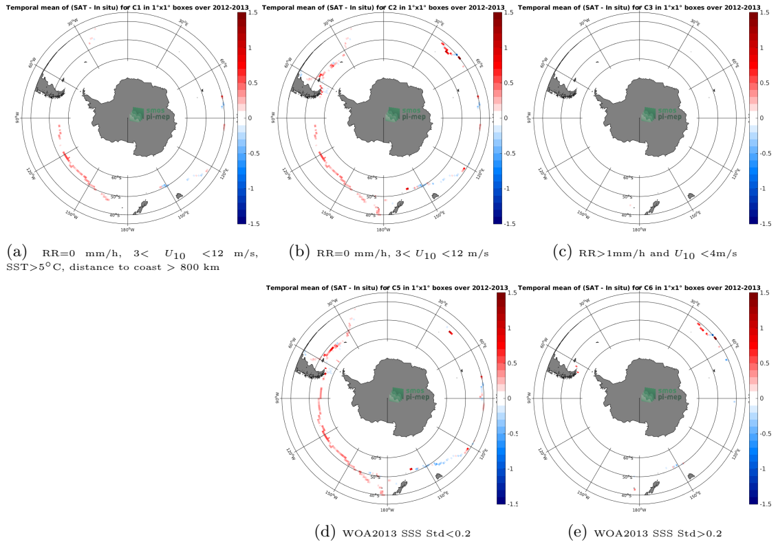
Figure 12: Temporal mean gridded over spatial boxes of size 1^\circ \times 1^\circ of \Delta SSS (Aquarius-L4-IPRC-V5-WEEKLY - TSG-GOSUD-Sailing-ship) for 5 different subdatasets corresponding to:RR=0 mm/h, 3 < U_{10} < 12 m/s, SST >5^\circ C, distance to coast > 800 km (a), RR=0 mm/h, 3 < U_{10} < 12 m/s (b), RR >1 mm/h and U_{10} < 4 m/s (c), WOA2013 SSS Std <0.2 (d), WOA2013 SSS Std >0.2 (e).
