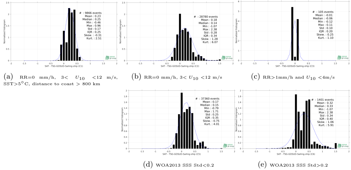
Figure 13: Normalized histogram of \Delta\text{SSS} (Aquarius-L4-IPRC-V5-WEEKLY - TSG-GOSUD-Sailing-ship) for 5 different subdatasets corresponding to: RR=0 mm/h, 3 < U_{10} < 12 m/s, SST > 5^{\circ}\text{C} , distance to coast > 800 km (a), RR=0 mm/h, 3 < U_{10} < 12 m/s (b), RR > 1\text{mm/h} and U_{10} < 4\text{m/s} (c), WOA2013 SSS Std < 0.2 (d), WOA2013 SSS Std > 0.2 (e).
