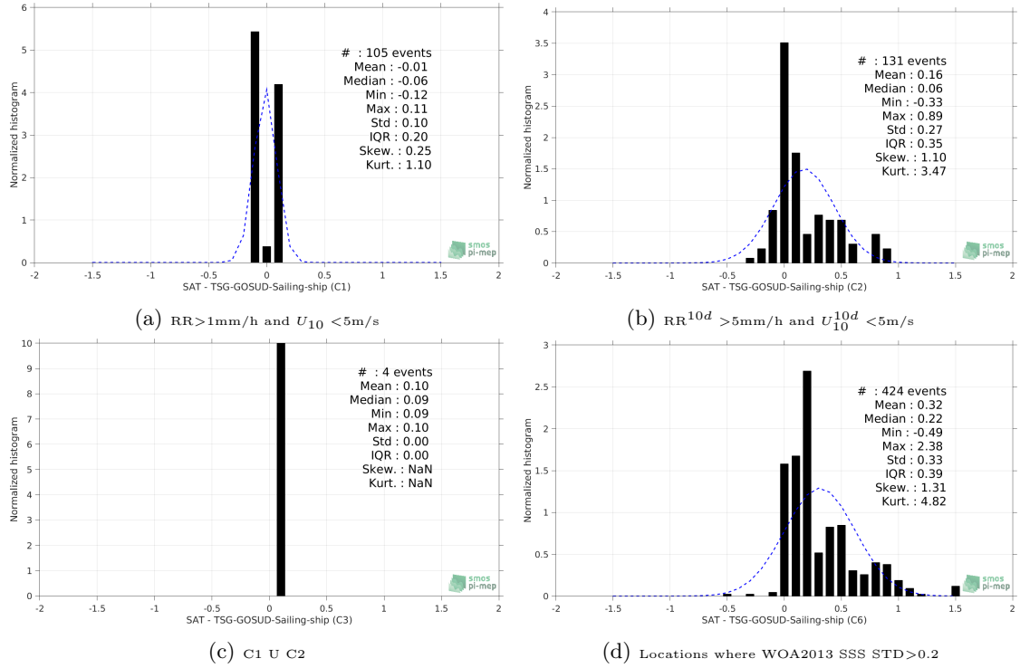
Figure 13: Normalized histogram of \Delta SSS (Aquarius-L4-IPRC-V5-WEEKLY - TSG-GOSUD-Sailing-ship) for 6 different subdatasets corresponding to: RR > 1\text{mm/h} and U_{10} < 5\text{m/s} (a), RR^{10d} > 5\text{mm/h} and U_{10}^{10d} < 5\text{m/s} (b), C1 U C2 (c), Locations where WOA2013 SSS STD > 0.2 (d).
