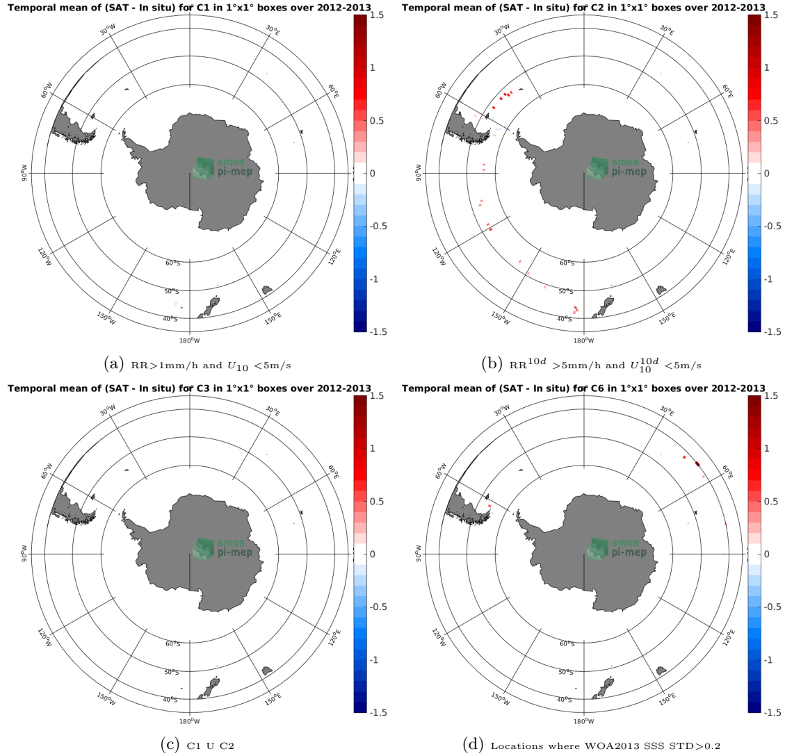
Figure 12: Temporal mean gridded over spatial boxes of size 1^\circ \times 1^\circ of \Delta SSS (Aquarius-L4-IPRC-V5-WEEKLY - TSG-GOSUD-Sailing-ship) for 4 different subdatasets corresponding to: RR > 1\text{mm/h} and U_{10} < 5\text{m/s} (a), RR^{10d} > 5\text{mm/h} and U_{10}^{10d} < 5\text{m/s} (b), C1 U C2 (c), Locations where WOA2013 SSS STD > 0.2 (d).
