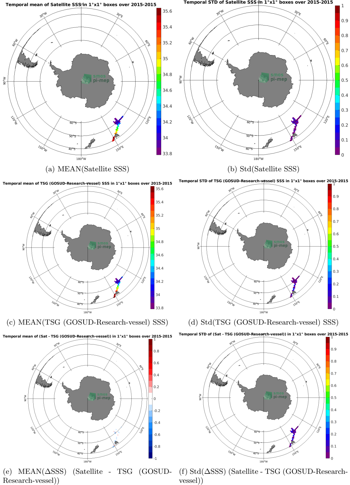
Figure 6: Temporal mean (left) and Std (right) of SSS from Aquarius SSS L4 OI v5 - Weekly (IPRC) (top), TSG (GOSUD-Research-vessel) (middle), and of \Delta SSS (Satellite - TSG (GOSUD-Research-vessel)). Only match-up pairs are used to generate these maps.
