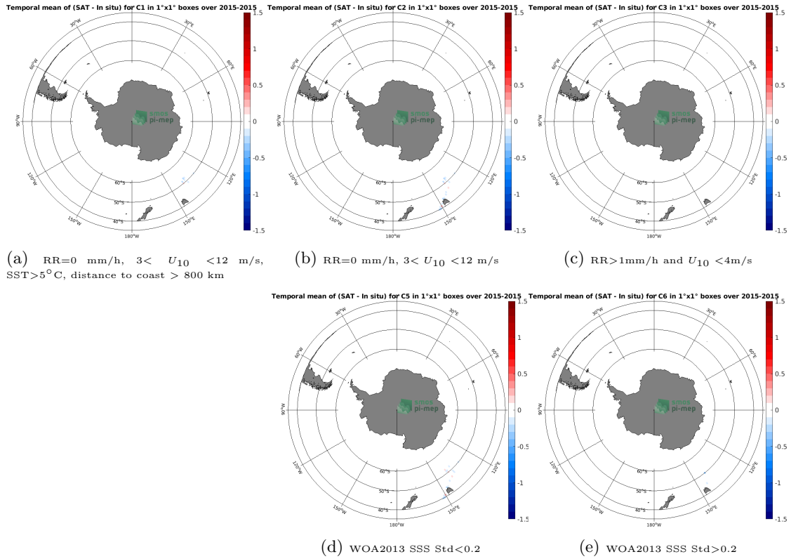
Figure 12: Temporal mean gridded over spatial boxes of size 1°×1° of \Delta SSS (Aquarius SSS L4 OI v5 - Weekly (IPRC) - TSG (GOSUD-Research-vessel)) for 5 different subdatasets corresponding to:RR=0 mm/h, 3 < U_{10} < 12 m/s, SST>5°C, distance to coast > 800 km (a), RR=0 mm/h, 3 < U_{10} < 12 m/s (b), RR>1mm/h and U_{10} < 4 m/s (c), WOA2013 SSS Std<0.2 (d), WOA2013 SSS Std>0.2 (e).
