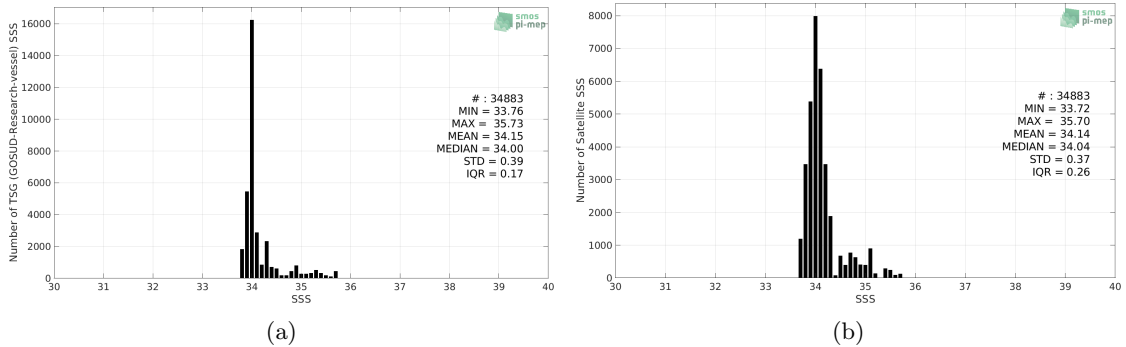
Figure 2: Histograms of SSS from TSG (GOSUD-Research-vessel) (a) and Aquarius SSS L4 OI v5 - Weekly (IPRC) (b) considering all match-up pairs per bins of 0.1 over the Roaring Forties and Furious Fifties Pi-MEP region and for the full satellite product period.
