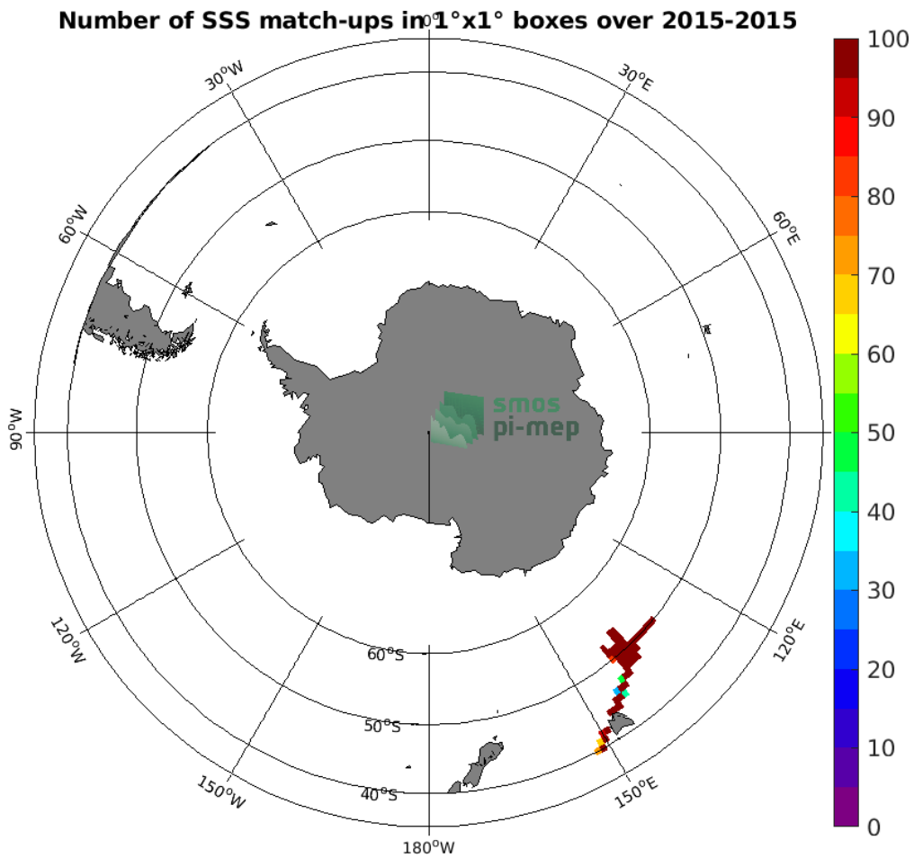
Figure 4: Number of SSS match-ups between TSG (GOSUD-Research-vessel) SSS and the Aquarius SSS L4 OI v5 - Weekly (IPRC) SSS product for the Roaring Forties and Furious Fifties Pi-MEP region over 1^\circ \times 1^\circ boxes and for the full satellite product period.
