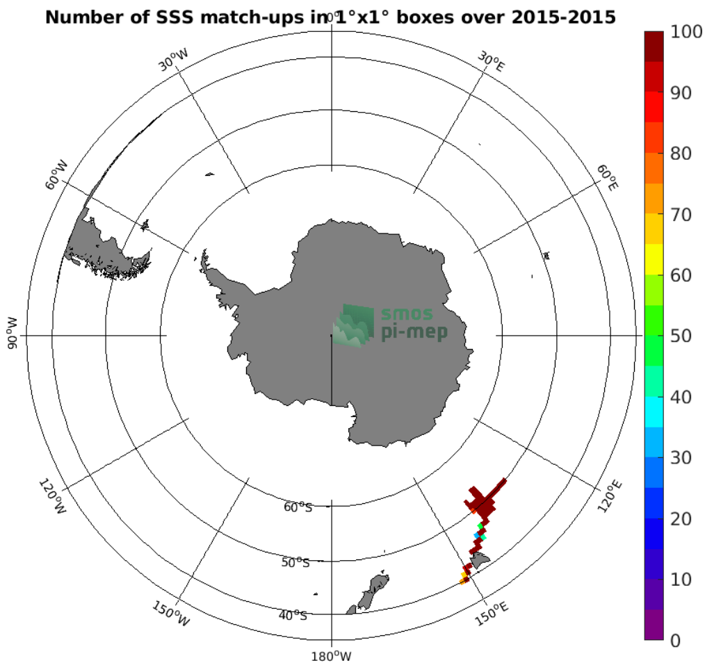
Figure 4: Number of SSS match-ups between TSG (GOSUD-Research-vessel) SSS and the Aquarius SSS L4 OI v5 - Weekly (IPRC) SSS product for the Roaring Forties and Furious Fifties Pi-MEP region over 1^{\circ} \times 1^{\circ} boxes and for the full satellite product period.
