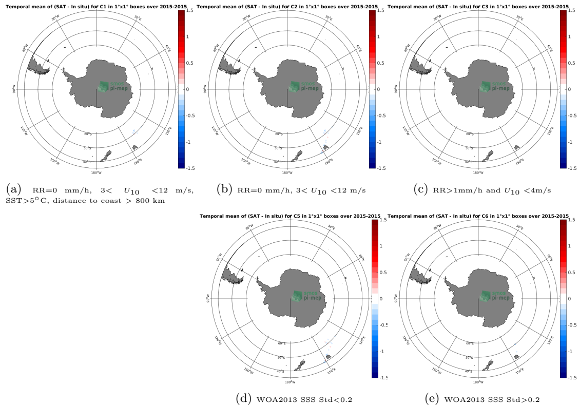
Figure 12: Temporal mean gridded over spatial boxes of size 1^\circ \times 1^\circ of \Delta SSS (Aquarius-L4-IPRC-V5-WEEKLY - TSG-GOSUD-Research-vessel) for 5 different subdatasets corresponding to: RR=0 mm/h, 3 < U_{10} < 12 m/s, SST > 5^\circ\text{C} , distance to coast > 800 km (a), RR=0 mm/h, 3 < U_{10} < 12 m/s (b), RR > 1 mm/h and U_{10} < 4 m/s (c), WOA2013 SSS Std < 0.2 (d), WOA2013 SSS Std > 0.2 (e).
