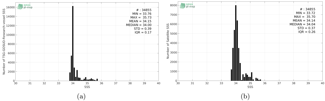
Figure 2: Histograms of SSS from TSG-GOSUD-Research-vessel (a) and Aquarius-L4-IPRC-V5-WEEKLY (b) considering all match-up pairs per bins of 0.1 over the Roaring Forties and Furious Fifties Pi-MEP region and for the full satellite product period.
