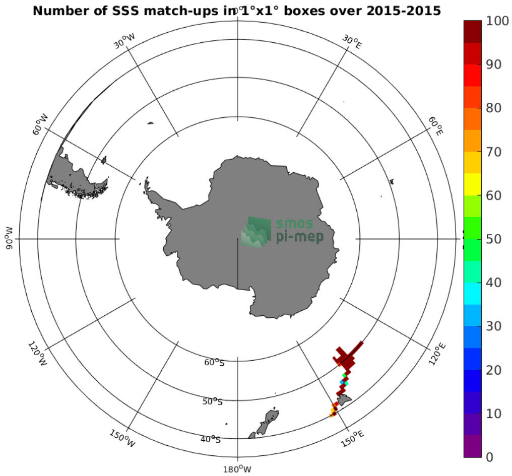
Figure 4: Number of SSS match-ups between TSG-GOSUD-Research-vessel SSS and the Aquarius-L4-IPRC-V5-WEEKLY SSS product for the Roaring Forties and Furious Fifties Pi-MEP region over 1°x1° boxes and for the full satellite product period.
