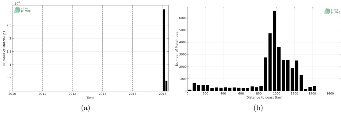
Figure 1: Number of match-ups between TSG-GOSUD-Research-vessel and Aquarius-L4-IPRC-V5-WEEKLY SSS as a function of time (a) and as function of the distance to coast (b) over the Roaring Forties and Furious Fifties Pi-MEP region and for the full satellite product period.
