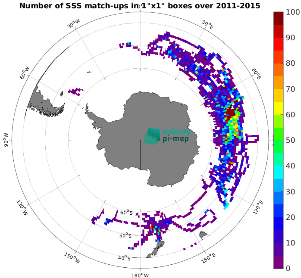
Figure 5: Number of SSS match-ups between Marine mammals SSS and the Aquarius SSS L4 OI v5 - Weekly (IPRC) SSS product for the Roaring Forties and Furious Fifties Pi-MEP region over 1^\circ \times 1^\circ boxes and for the full satellite product period.
