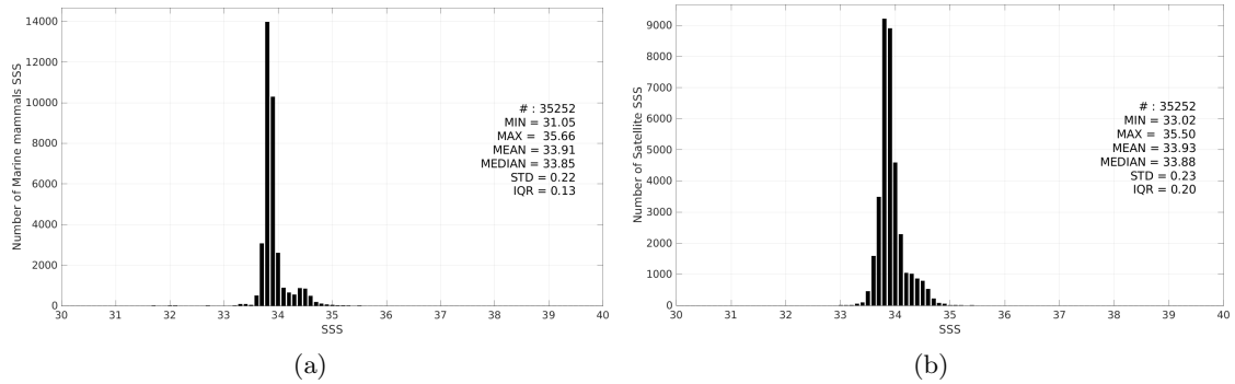
Figure 3: Histograms of SSS from Marine mammals (a) and Aquarius SSS L4 OI v5 - Weekly (IPRC) (b) considering all match-up pairs per bins of 0.1 over the Roaring Forties and Furious Fifties Pi-MEP region and for the full satellite product period.
