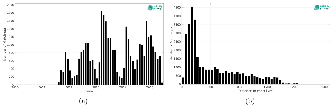
Figure 2: Number of match-ups between Marine mammals and Aquarius SSS L4 OI v5 - Weekly (IPRC) SSS as a function of time (a) and as function of the distance to coast (b) over the Roaring Forties and Furious Fifties Pi-MEP region and for the full satellite product period.
