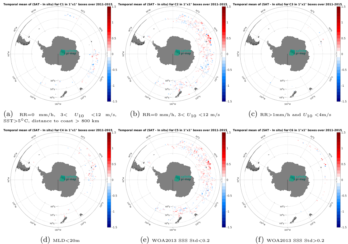
Figure 14: Temporal mean gridded over spatial boxes of size 1^\circ \times 1^\circ of \Delta SSS (Aquarius SSS L4 OI v5 - Weekly (IPRC) - Marine mammals) for 6 different subdatasets corresponding to:RR=0 mm/h, 3 < U_{10} < 12 m/s, SST>5°C, distance to coast > 800 km (a), RR=0 mm/h, 3 < U_{10} < 12 m/s (b), RR>1mm/h and U_{10} < 4 m/s (c),MLD<20m (d),WOA2013 SSS Std<0.2 (e),WOA2013 SSS Std>0.2 (f).
