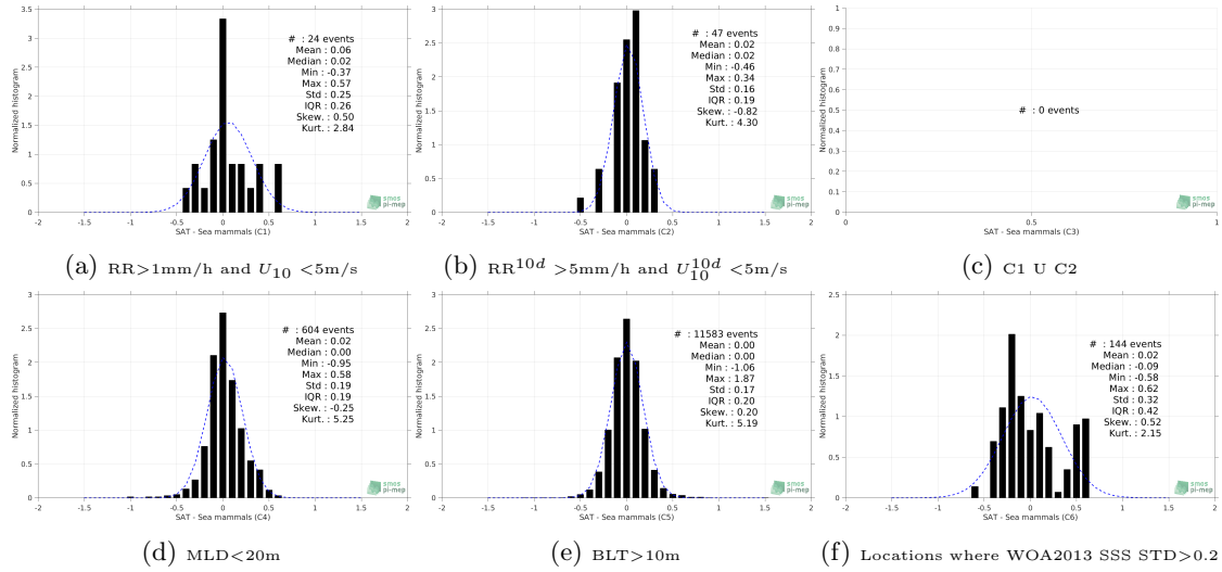
Figure 13: Normalized histogram of \Delta SSS (Aquarius-L4-IPRC-V5-WEEKLY - Sea mammals) for 6 different subdatasets corresponding to: RR>1mm/h and U_{10} < 5\text{m/s} (a), RR 10d >5mm/h and U_{10}^{10d} < 5\text{m/s} (b), C1 U C2 (c), MLD<20m (d), BLT>10m (e), Locations where WOA2013 SSS STD>0.2 (f).
