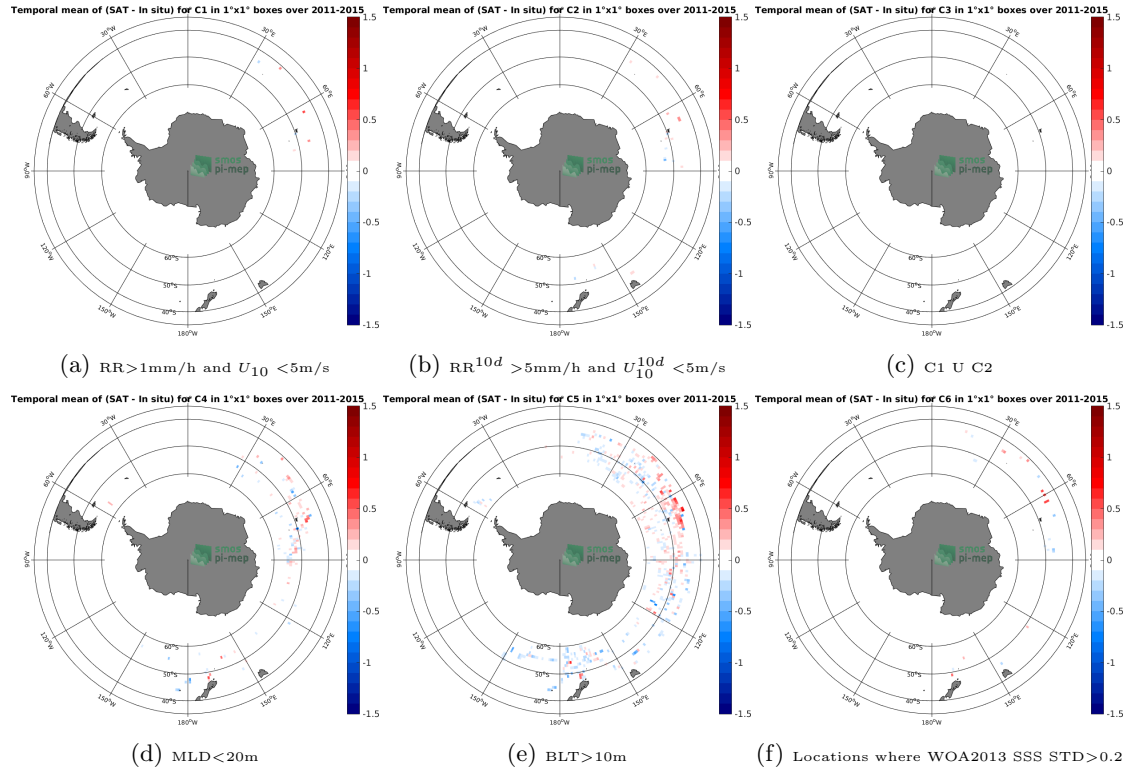
Figure 12: Temporal mean gridded over spatial boxes of size 1^\circ \times 1^\circ of \Delta\text{SSS} (Aquarius-L4-IPRC-V5-WEEKLY - Sea mammals) for 6 different subdatasets corresponding to: \text{RR} > 1\text{mm/h} and U_{10} < 5\text{m/s} (a), \text{RR}^{10d} > 5\text{mm/h} and U_{10}^{10d} < 5\text{m/s} (b), C1 U C2 (c), \text{MLD} < 20\text{m} (d), \text{BLT} > 10\text{m} (e), Locations where WOA2013 SSS STD > 0.2 (f).
