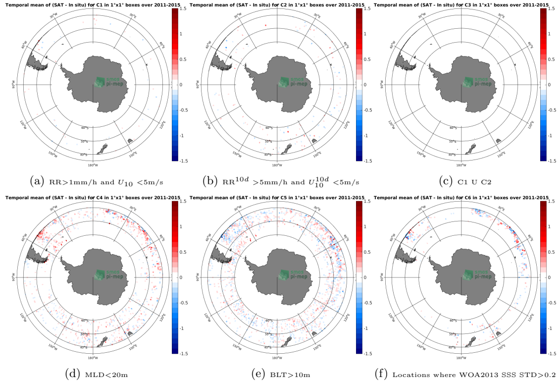
Figure 12: Temporal mean gridded over spatial boxes of size 1^\circ \times 1^\circ of \Delta SSS (Aquarius-L4-IPRC-V5-WEEKLY - Argo) for 6 different subdatasets corresponding to: RR > 1\text{mm/h} and U_{10} < 5\text{m/s} (a), RR^{10d} > 5\text{mm/h} and U_{10}^{10d} < 5\text{m/s} (b), C1 U C2 (c), MLD < 20\text{m} (d), BLT > 10\text{m} (e), Locations where WOA2013 SSS STD > 0.2 (f).
