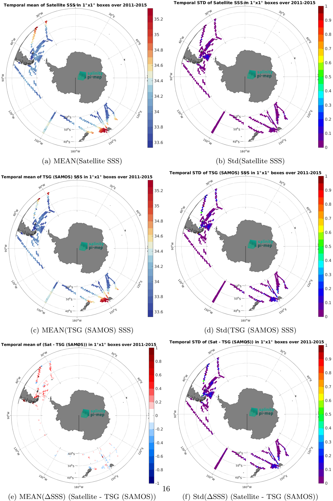
Figure 7: Temporal mean (left) and Std (right) of SSS from Aquarius SSS L4 OI v5 - Monthly (IPRC) (top), TSG (SAMOS) (middle), and of \Delta SSS (Satellite - TSG (SAMOS)). Only match-up pairs are used to generate these maps.
