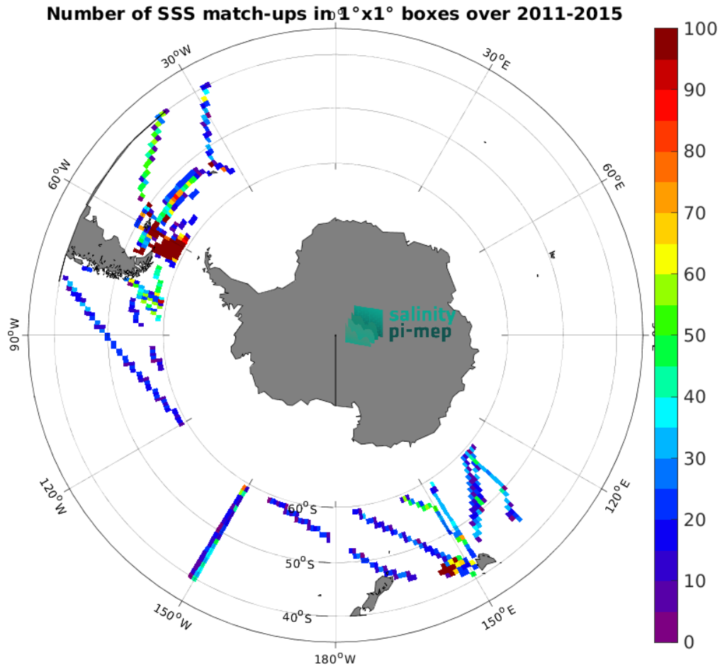
Figure 5: Number of SSS match-ups between TSG (SAMOS) SSS and the Aquarius SSS L4 OI v5 - Monthly (IPRC) SSS product for the Roaring Forties and Furious Fifties Pi-MEP region over 1^\circ \times 1^\circ boxes and for the full satellite product period.
