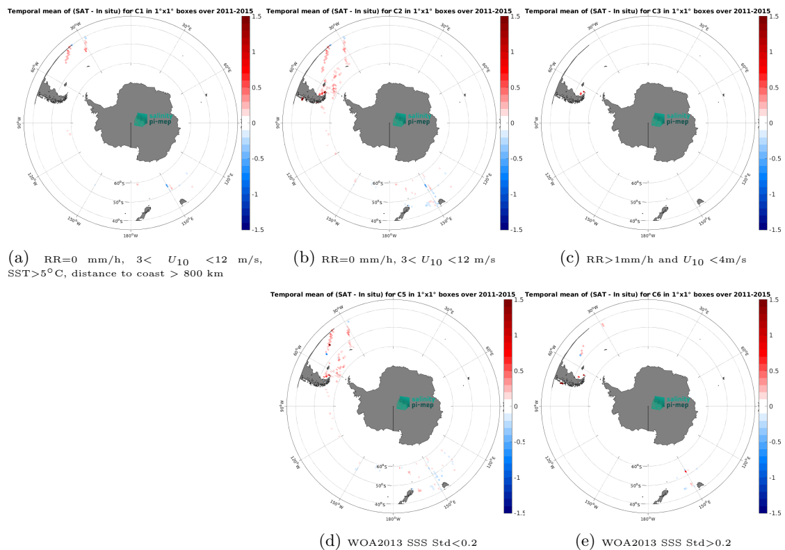
Figure 14: Temporal mean gridded over spatial boxes of size 1^\circ \times 1^\circ of \Delta SSS (Aquarius SSS L4 OI v5 - Monthly (IPRC) - TSG (SAMOS)) for 5 different subdatasets corresponding to:RR=0 mm/h, 3 < U_{10} < 12 m/s, SST>5°C, distance to coast > 800 km (a), RR=0 mm/h, 3 < U_{10} < 12 m/s (b), RR>1mm/h and U_{10} < 4 m/s (c), WOA2013 SSS Std<0.2 (d), WOA2013 SSS Std>0.2 (e).
