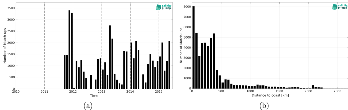
Figure 2: Number of match-ups between TSG (SAMOS) and Aquarius SSS L4 OI v5 - Monthly (IPRC) SSS as a function of time (a) and as function of the distance to coast (b) over the Roaring Forties and Furious Fifties Pi-MEP region and for the full satellite product period.
