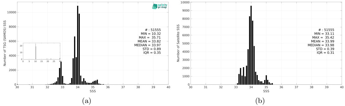
Figure 3: Histograms of SSS from TSG (SAMOS) (a) and Aquarius SSS L4 OI v5 - Monthly (IPRC) (b) considering all match-up pairs per bins of 0.1 over the Roaring Forties and Furious Fifties Pi-MEP region and for the full satellite product period.
