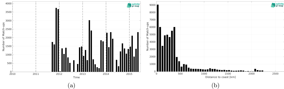
Figure 1: Number of match-ups between TSG (SAMOS) and Aquarius SSS L4 OI v5 - Monthly (IPRC) SSS as a function of time (a) and as function of the distance to coast (b) over the Roaring Forties and Furious Fifties Pi-MEP region and for the full satellite product period.
