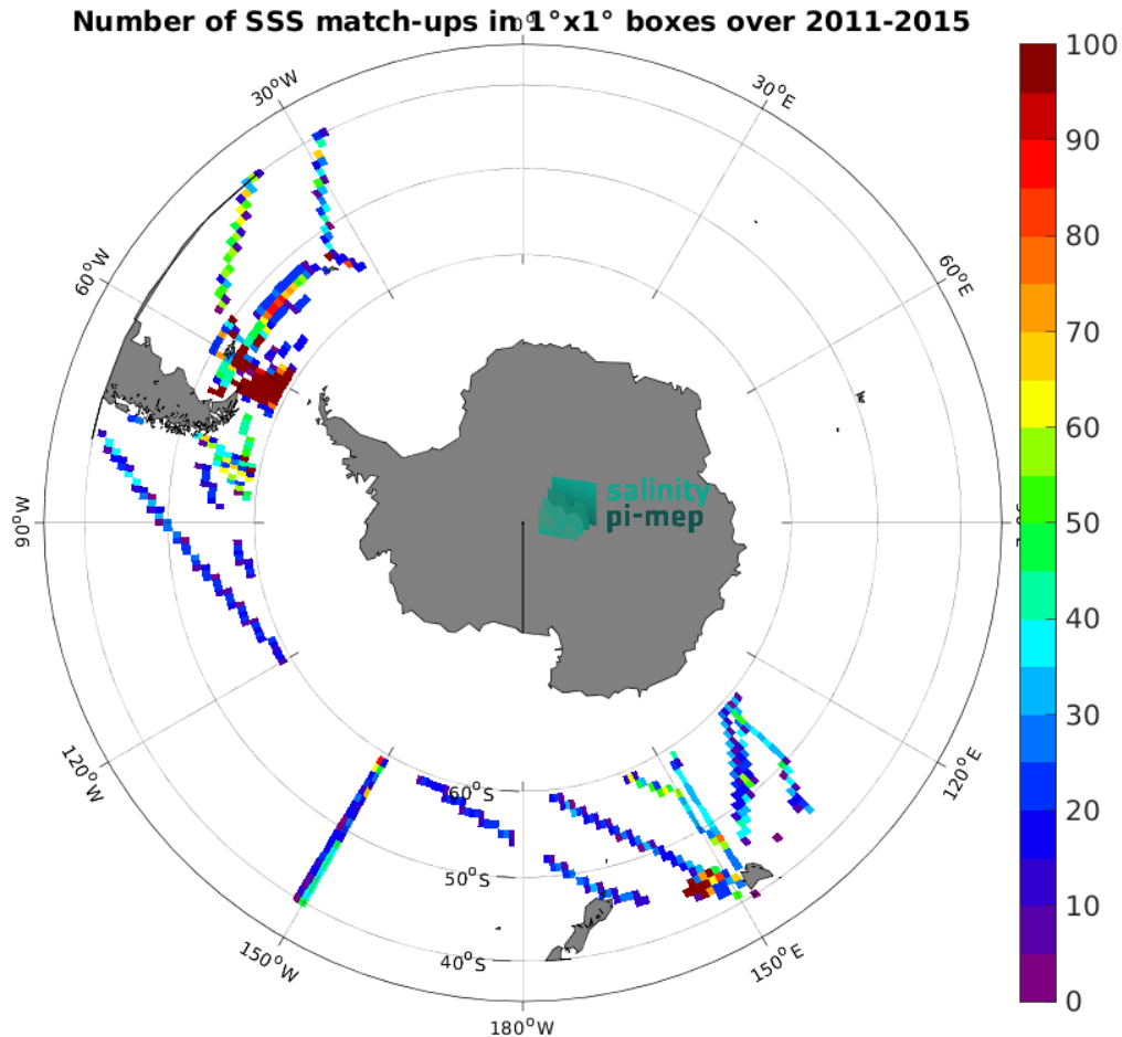
Figure 4: Number of SSS match-ups between TSG (SAMOS) SSS and the Aquarius SSS L4 OI v5 - Monthly (IPRC) SSS product for the Roaring Forties and Furious Fifties Pi-MEP region over 1^\circ \times 1^\circ boxes and for the full satellite product period.
