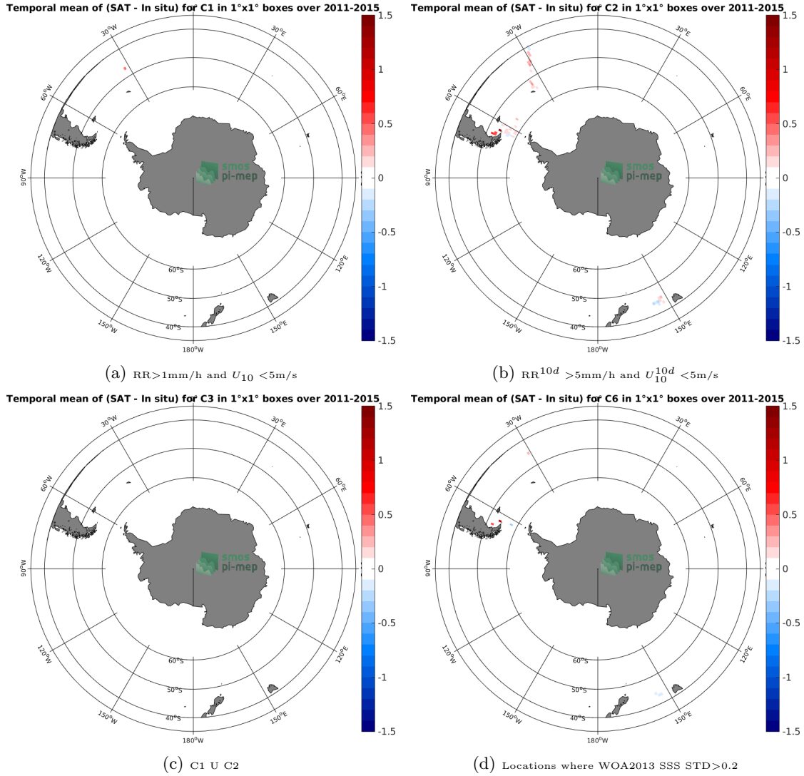
Figure 12: Temporal mean gridded over spatial boxes of size 1^\circ \times 1^\circ of \Delta SSS (Aquarius-L4-IPRC-V5-MONTHLY - TSG-SAMOS) for 4 different subdatasets corresponding to: RR > 1mm/h and U_{10} < 5\text{m/s} (a), RR^{10d} > 5\text{mm/h} and U_{10}^{10d} < 5\text{m/s} (b), C1 U C2 (c), Locations where WOA2013 SSS STD > 0.2 (d).
