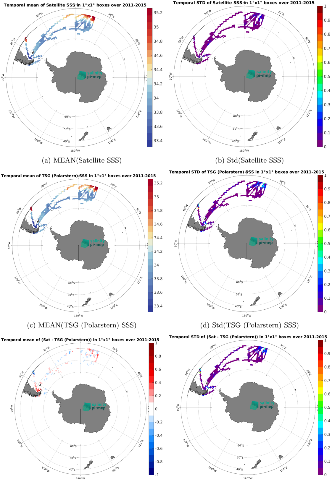
(e) MEAN( \Delta SSS) (Satellite - TSG (Polarstern)) 16 (f) Std( \Delta SSS) (Satellite - TSG (Polarstern)) Figure 7: Temporal mean (left) and Std (right) of SSS from Aquarius SSS L4 OI v5 - Monthly (IPRC) (top), TSG (Polarstern) (middle), and of \Delta SSS (Satellite - TSG (Polarstern)). Only match-up pairs are used to generate these maps.
