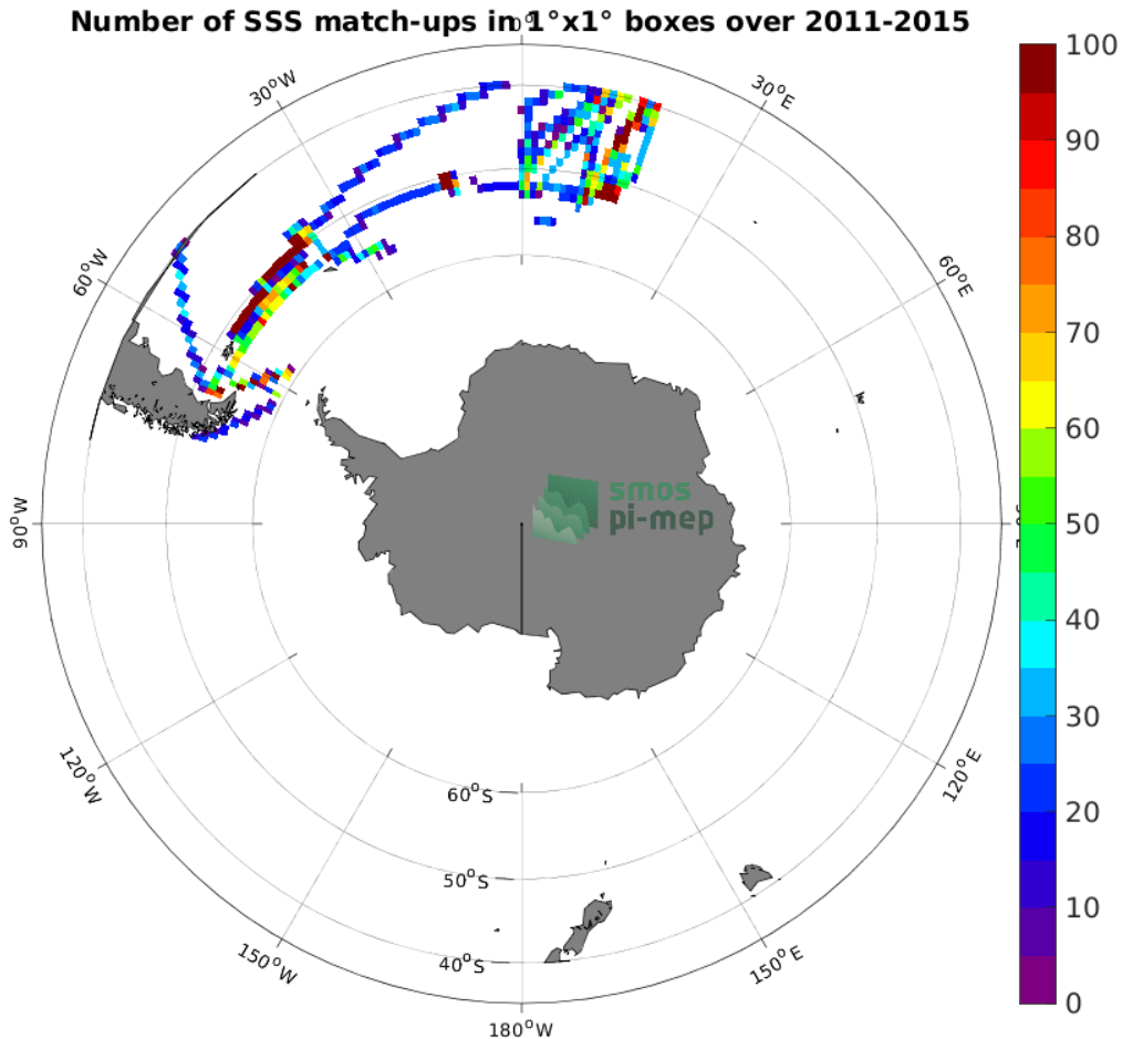
Figure 4: Number of SSS match-ups between TSG (Polarstern) SSS and the Aquarius SSS L4 OI v5 - Monthly (IPRC) SSS product for the Roaring Forties and Furious Fifties Pi-MEP region over 1^\circ \times 1^\circ boxes and for the full satellite product period.
