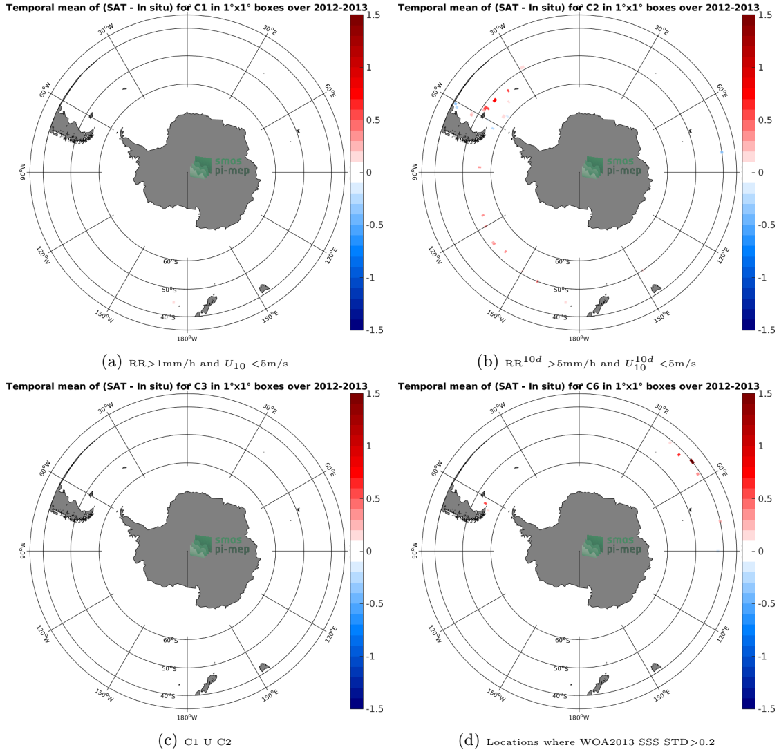
Figure 12: Temporal mean gridded over spatial boxes of size 1^\circ \times 1^\circ of \Delta SSS (Aquarius-L4-IPRC-V5-MONTHLY - TSG-GOSUD-Sailing-ship) for 4 different subdatasets corresponding to: RR > 1\text{mm/h} and U_{10} < 5\text{m/s} (a), RR^{10d} > 5\text{mm/h} and U_{10}^{10d} < 5\text{m/s} (b), C1 U C2 (c), Locations where WOA2013 SSS STD > 0.2 (d).
