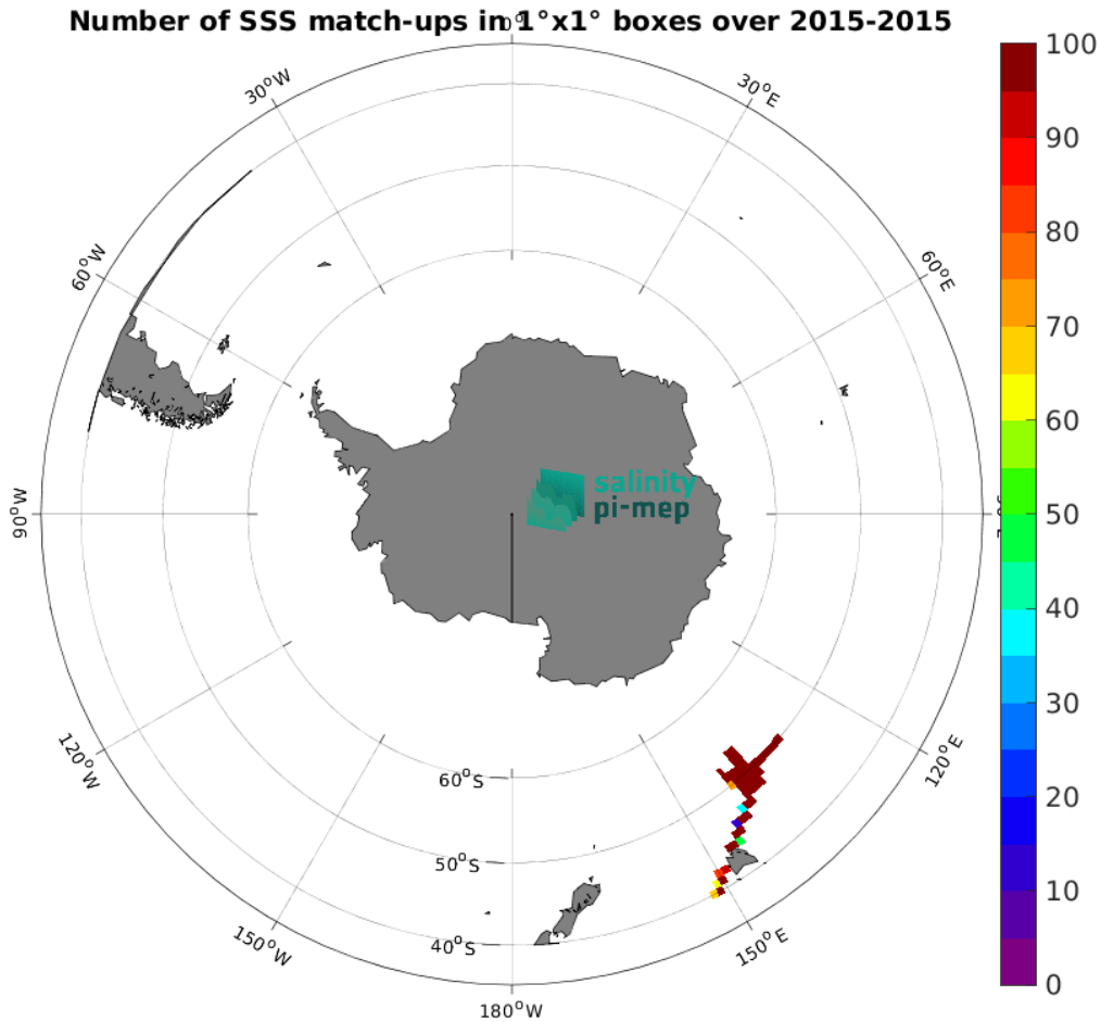
Figure 5: Number of SSS match-ups between TSG (GOSUD-Research-vessel) SSS and the Aquarius SSS L4 OI v5 - Monthly (IPRC) SSS product for the Roaring Forties and Furious Fifties Pi-MEP region over 1^\circ \times 1^\circ boxes and for the full satellite product period.
