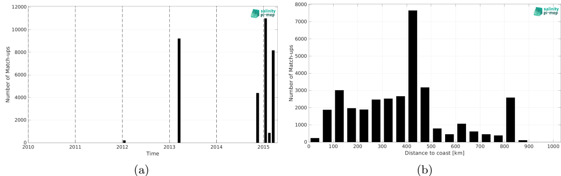
Figure 2: Number of match-ups between TSG (CSIC-UTM) and Aquarius SSS L4 OI v5 - Monthly (IPRC) SSS as a function of time (a) and as function of the distance to coast (b) over the Roaring Forties and Furious Fifties Pi-MEP region and for the full satellite product period.
