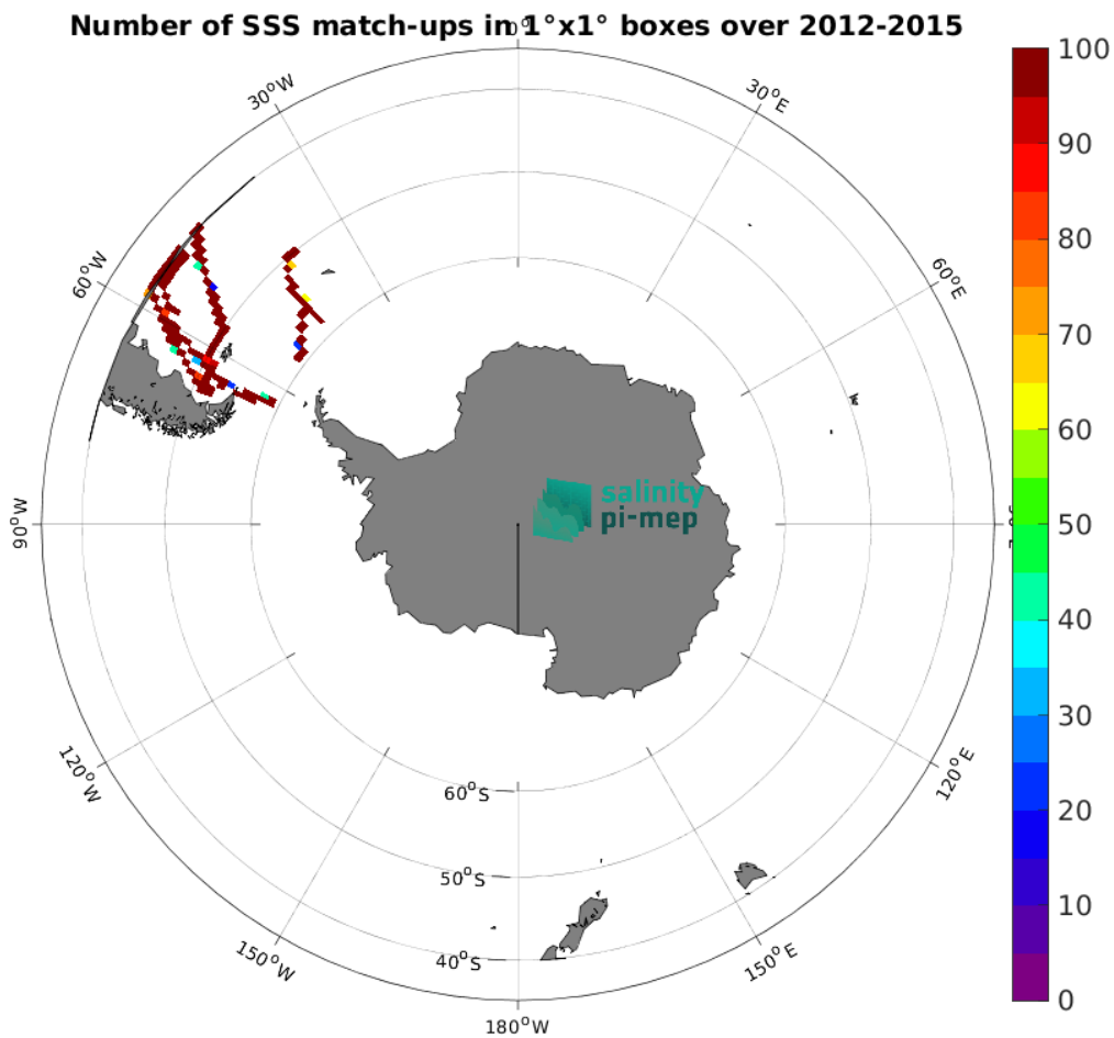
Figure 5: Number of SSS match-ups between TSG (CSIC-UTM) SSS and the Aquarius SSS L4 OI v5 - Monthly (IPRC) SSS product for the Roaring Forties and Furious Fifties Pi-MEP region over 1^\circ \times 1^\circ boxes and for the full satellite product period.
