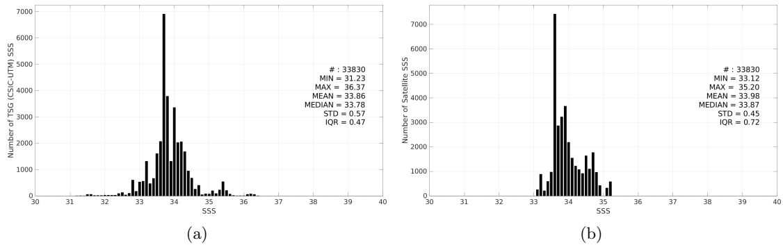
Figure 3: Histograms of SSS from TSG (CSIC-UTM) (a) and Aquarius SSS L4 OI v5 - Monthly (IPRC) (b) considering all match-up pairs per bins of 0.1 over the Roaring Forties and Furious Fifties Pi-MEP region and for the full satellite product period.
