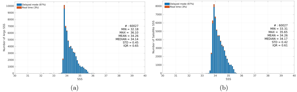
Figure 3: Histograms of SSS from Argo (a) and Aquarius SSS L4 OI v5 - Monthly (IPRC) (b) considering all match-up pairs per bins of 0.1 over the Roaring Forties and Furious Fifties Pi-MEP region and for the full satellite product period.
