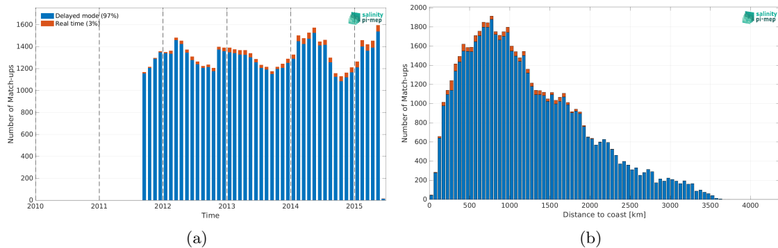
Figure 2: Number of match-ups between Argo and Aquarius SSS L4 OI v5 - Monthly (IPRC) SSS as a function of time (a) and as function of the distance to coast (b) over the Roaring Forties and Furious Fifties Pi-MEP region and for the full satellite product period.
