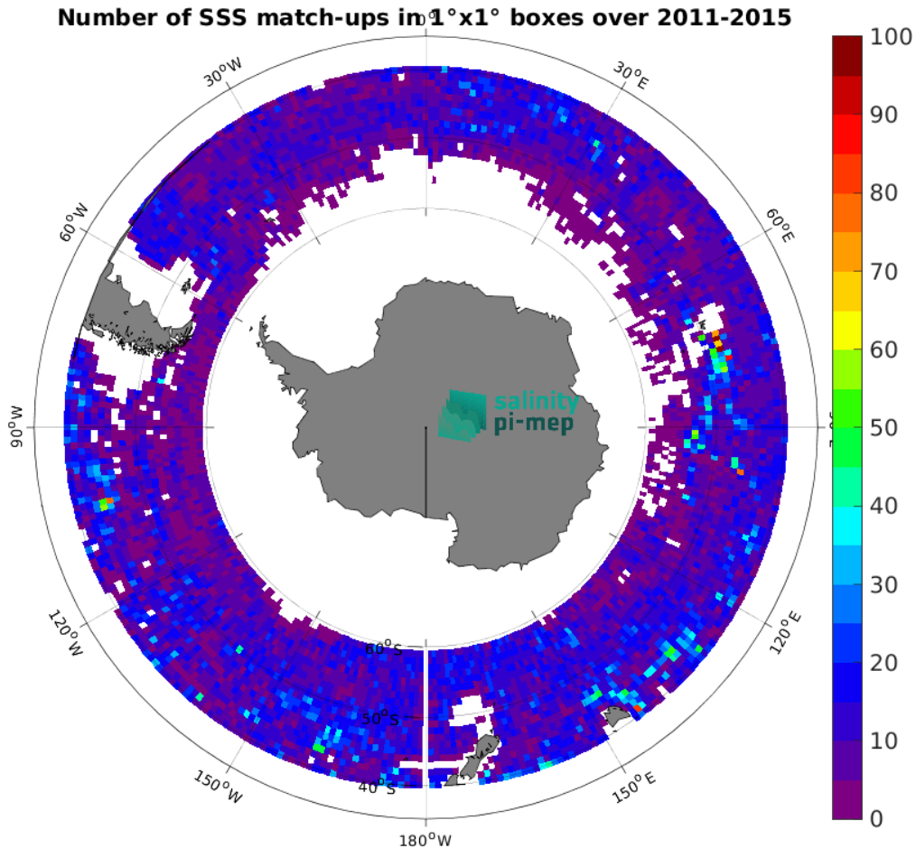
Figure 5: Number of SSS match-ups between Argo SSS and the Aquarius SSS L4 OI v5 - Monthly (IPRC) SSS product for the Roaring Forties and Furious Fifties Pi-MEP region over 1^\circ \times 1^\circ boxes and for the full satellite product period.
