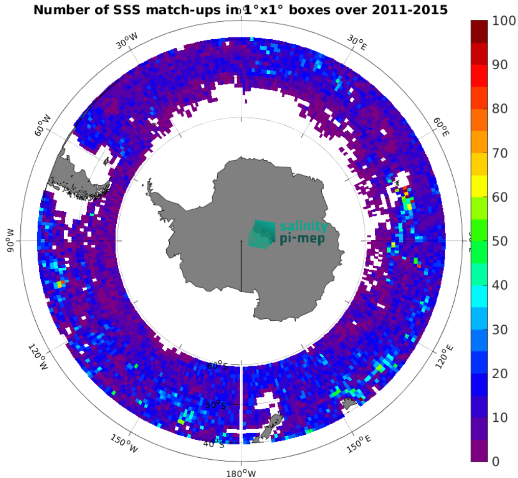
Figure 4: Number of SSS match-ups between Argo SSS and the Aquarius SSS L4 OI v5 - Monthly (IPRC) SSS product for the Roaring Forties and Furious Fifties Pi-MEP region over 1^\circ \times 1^\circ boxes and for the full satellite product period.
