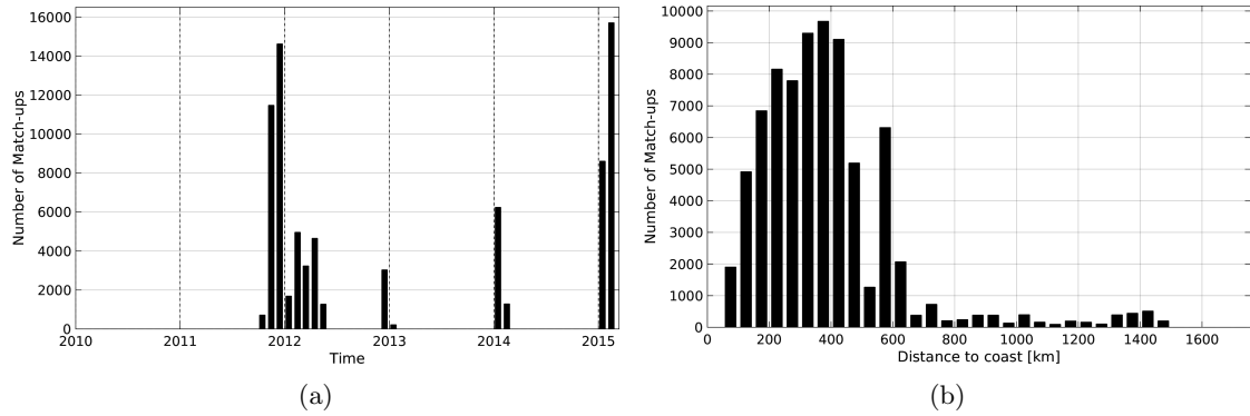
Figure 1: Number of match-ups between TSG-SAMOS and Aquarius-L4-IPRC-V4-WEEKLY SSS as a function of time (a) and as function of the distance to coast (b) over the Roaring Forties and Furious Fifties Pi-MEP region and for the full satellite product period.
