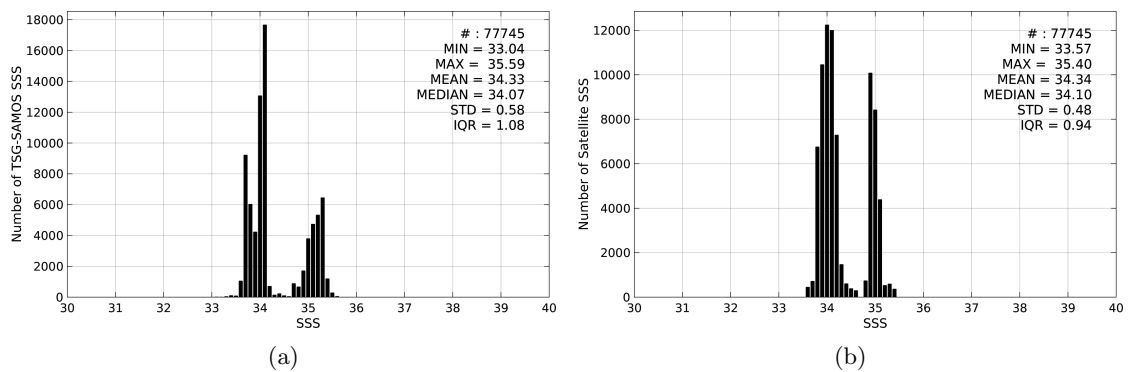
Figure 2: Histograms of SSS from TSG-SAMOS (a) and Aquarius-L4-IPRC-V4-WEEKLY (b) considering all match-up pairs per bins of 0.1 over the Roaring Forties and Furious Fifties Pi-MEP region and for the full satellite product period.
