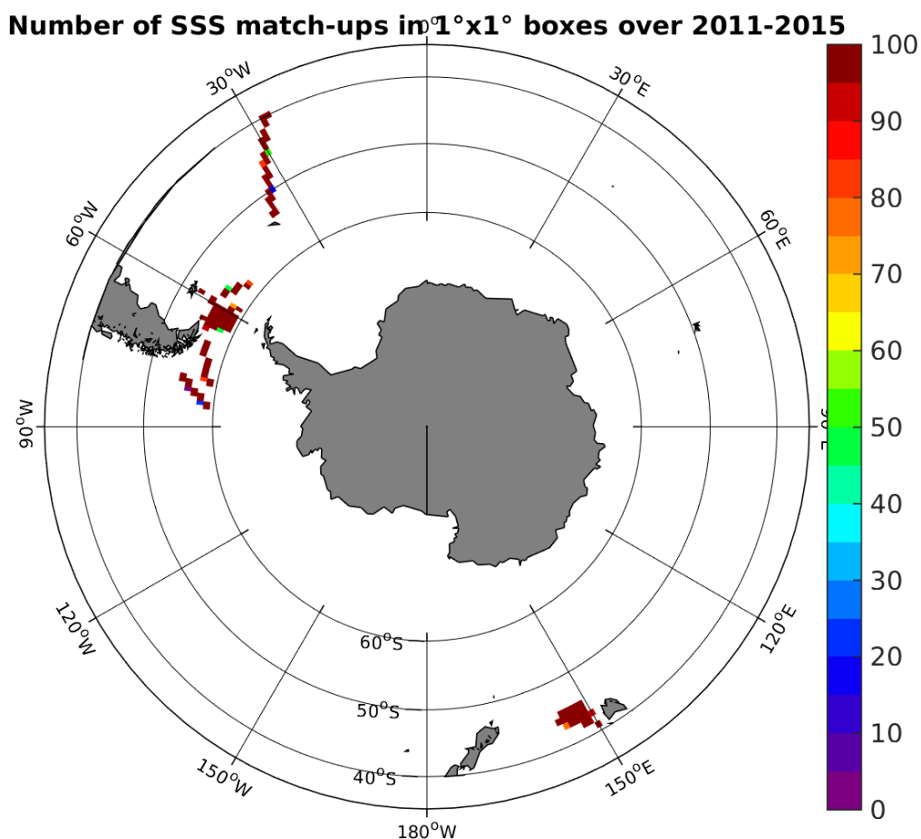
Figure 4: Number of SSS match-ups between TSG-SAMOS SSS and the Aquarius-L4-IPRC-V4-WEEKLY SSS product for the Roaring Forties and Furious Fifties Pi-MEP region over 1°x1° boxes and for the full satellite product period.
