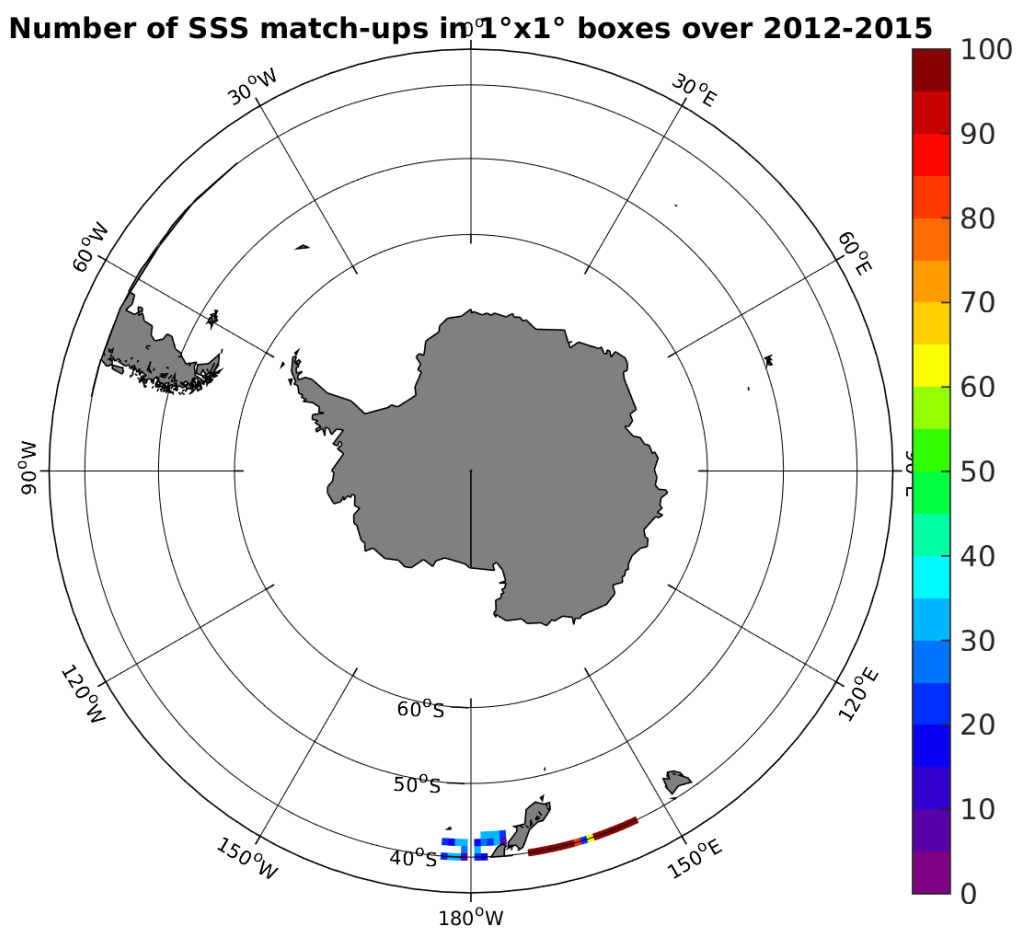
Figure 4: Number of SSS match-ups between TSG-LEGOS-DM SSS and the Aquarius-L4-IPRC-V4-WEEKLY SSS product for the Roaring Forties and Furious Fifties Pi-MEP region over 1^\circ \times 1^\circ boxes and for the full satellite product period.
