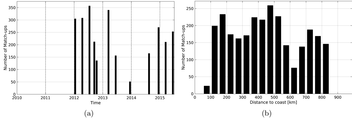
Figure 1: Number of match-ups between TSG-LEGOS-DM and Aquarius-L4-IPRC-V4-WEEKLY SSS as a function of time (a) and as function of the distance to coast (b) over the Roaring Forties and Furious Fifties Pi-MEP region and for the full satellite product period.
