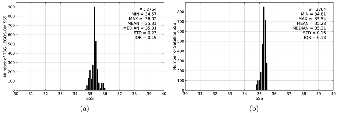
Figure 2: Histograms of SSS from TSG-LEGOS-DM (a) and Aquarius-L4-IPRC-V4-WEEKLY (b) considering all match-up pairs per bins of 0.1 over the Roaring Forties and Furious Fifties Pi-MEP region and for the full satellite product period.
