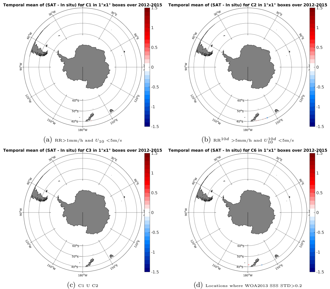
Figure 12: Temporal mean gridded over spatial boxes of size 1^\circ \times 1^\circ of \Delta SSS (Aquarius-L4-IPRC-V4-WEEKLY - TSG-LEGOS-DM) for 4 different subdatasets corresponding to: RR > 1\text{mm/h} and U_{10} < 5\text{m/s} (a), RR^{10d} > 5\text{mm/h} and U_{10}^{10d} < 5\text{m/s} (b), C1 U C2 (c), Locations where WOA2013 SSS STD > 0.2 (d).
