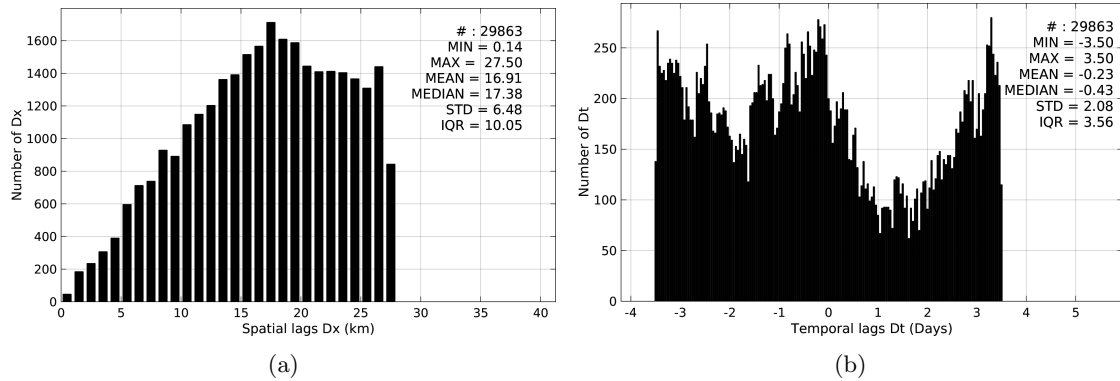
Figure 5: Histograms of the spatial (a) and temporal (b) lags between the time of the TSG-GOSUD-Sailing-ship measurements and the date of the corresponding Aquarius-L4-IPRC-V4-WEEKLY SSS product.
