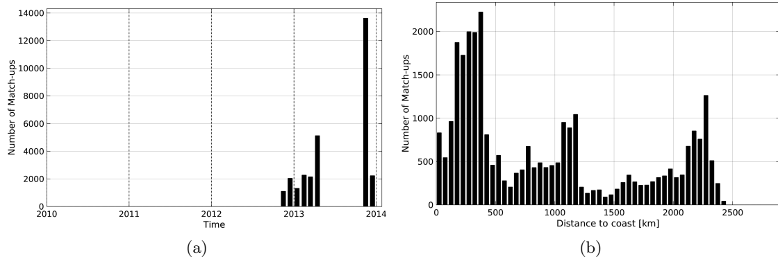
Figure 1: Number of match-ups between TSG-GOSUD-Sailing-ship and Aquarius-L4-IPRC-V4-WEEKLY SSS as a function of time (a) and as function of the distance to coast (b) over the Roaring Forties and Furious Fifties Pi-MEP region and for the full satellite product period.
