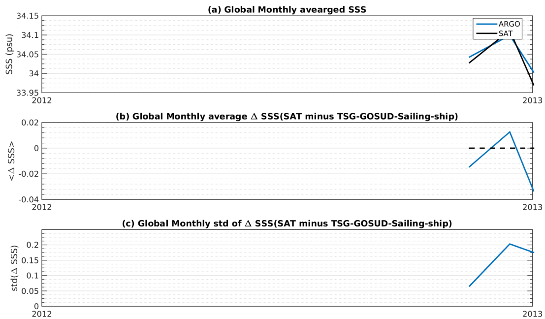
Figure 7: Time series of the monthly averaged mean SSS (top), mean \Delta SSS (Satellite - TSG-GOSUD-Sailing-ship) and STD of \Delta SSS (Satellite - TSG-GOSUD-Sailing-ship) over the Roaring Forties and Furious Fifties Pi-MEP region considering all match-ups collected by the Pi-MEP platform.
