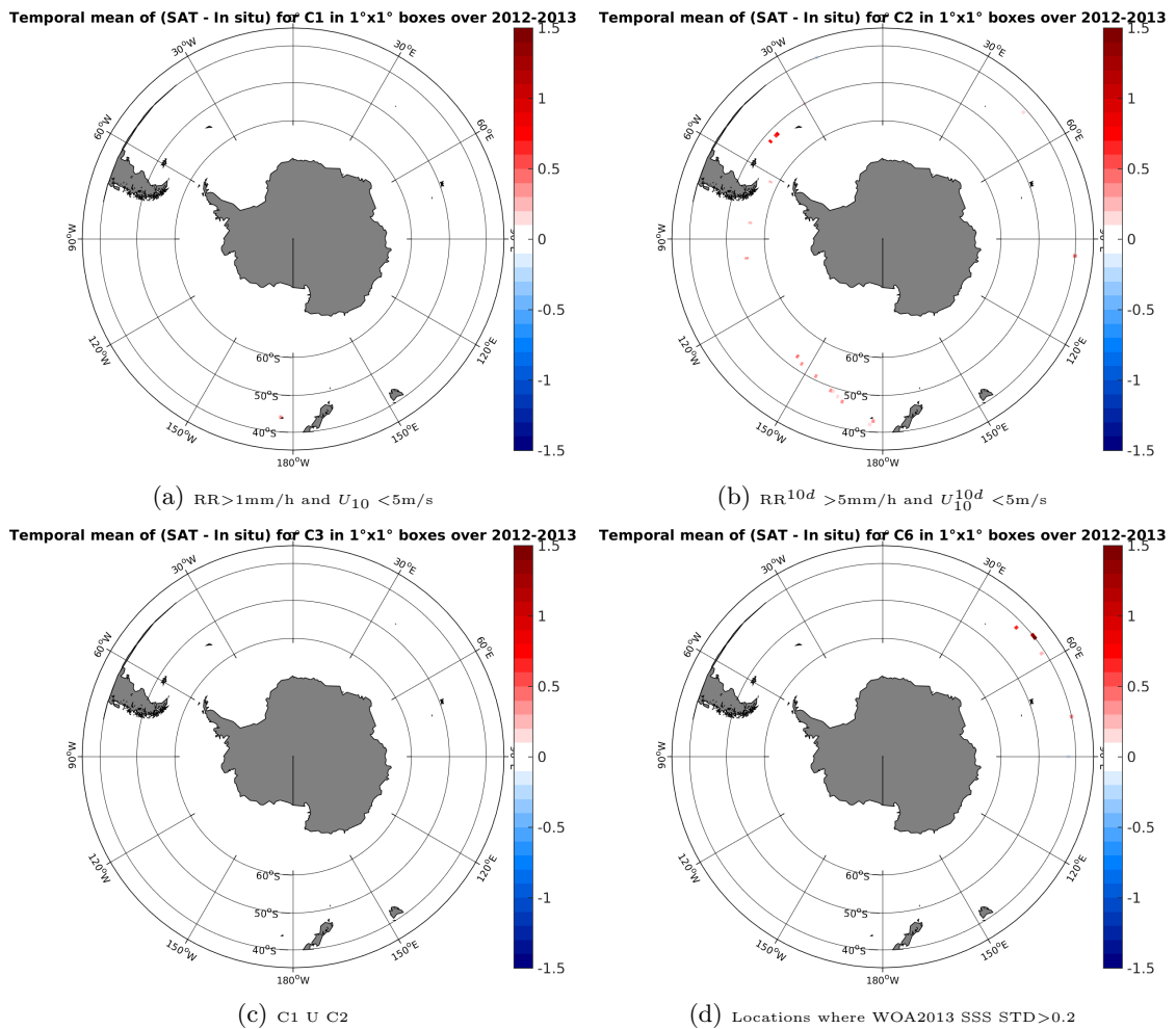
Figure 12: Temporal mean gridded over spatial boxes of size 1^\circ \times 1^\circ of \Delta SSS (Aquarius-L4-IPRC-V4-WEEKLY - TSG-GOSUD-Sailing-ship) for 4 different subdatasets corresponding to: RR > 1\text{mm/h} and U_{10} < 5\text{m/s} (a), RR^{10d} > 5\text{mm/h} and U_{10}^{10d} < 5\text{m/s} (b), C1 U C2 (c), Locations where WOA2013 SSS STD > 0.2 (d).
