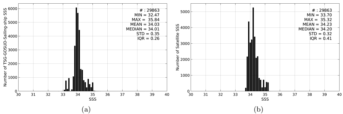
Figure 2: Histograms of SSS from TSG-GOSUD-Sailing-ship (a) and Aquarius-L4-IPRC-V4-WEEKLY (b) considering all match-up pairs per bins of 0.1 over the Roaring Forties and Furious Fifties Pi-MEP region and for the full satellite product period.
