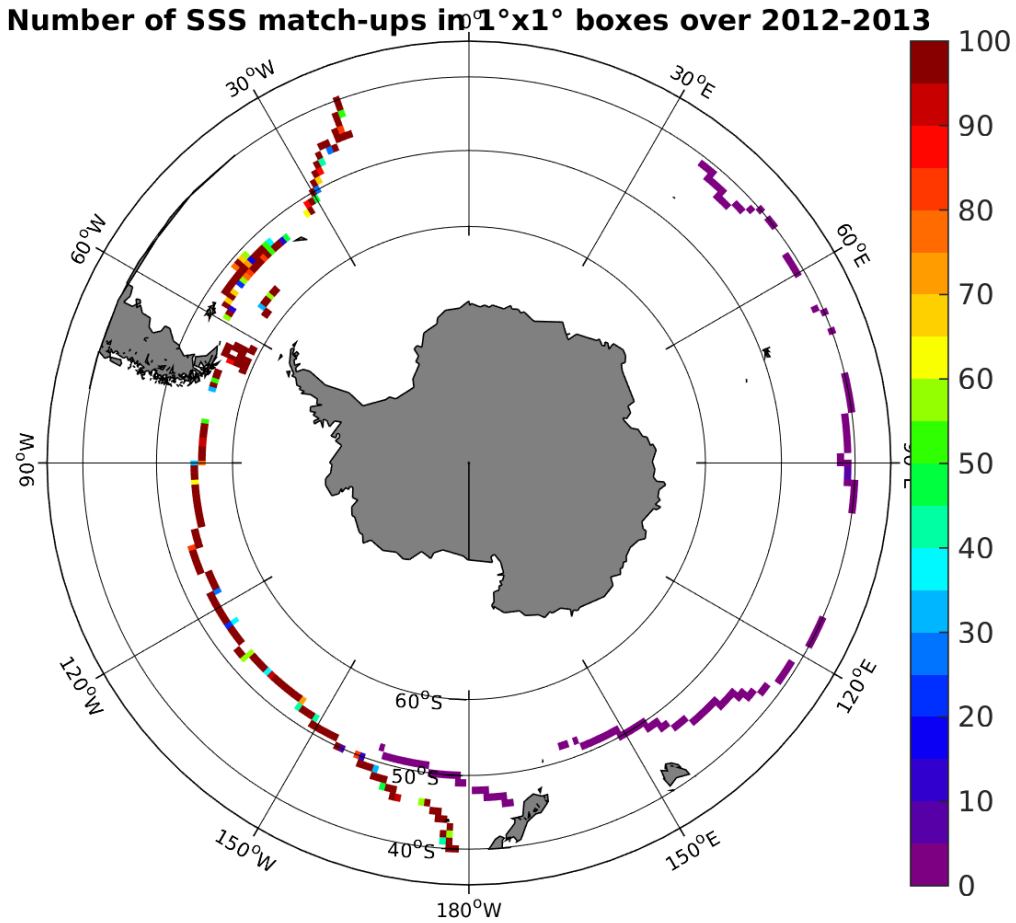
Figure 4: Number of SSS match-ups between TSG-GOSUD-Sailing-ship SSS and the Aquarius-L4-IPRC-V4-WEEKLY SSS product for the Roaring Forties and Furious Fifties Pi-MEP region over 1^\circ \times 1^\circ boxes and for the full satellite product period.
