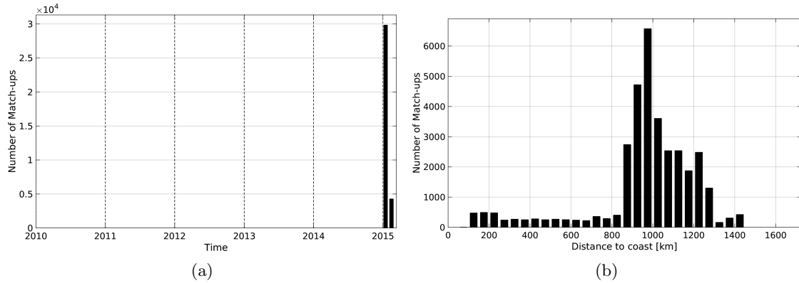
Figure 1: Number of match-ups between TSG-GOSUD-Research-vessel and Aquarius-L4-IPRC-V4-WEEKLY SSS as a function of time (a) and as function of the distance to coast (b) over the Roaring Forties and Furious Fifties Pi-MEP region and for the full satellite product period.
