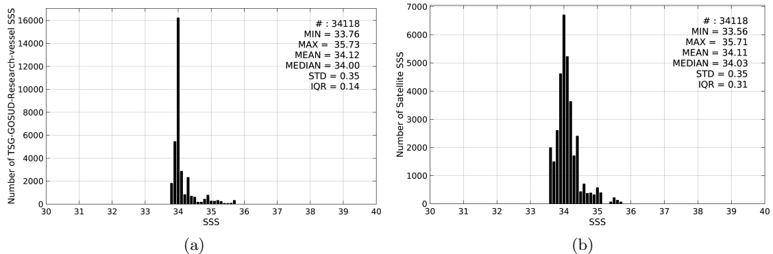
Figure 2: Histograms of SSS from TSG-GOSUD-Research-vessel (a) and Aquarius-L4-IPRC-V4-WEEKLY (b) considering all match-up pairs per bins of 0.1 over the Roaring Forties and Furious Fifties Pi-MEP region and for the full satellite product period.
