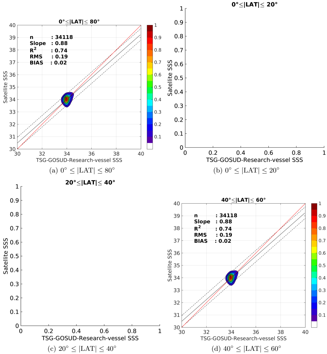
Figure 9: Contour maps of the concentration of Aquarius-L4-IPRC-V4-WEEKLY SSS (y-axis) versus TSG-GOSUD-Research-vessel SSS (x-axis) at match-up pairs for different latitude bands. For each plot, the red line shows x=y . The black thin and dashed lines indicate a linear fit through the data cloud and the \pm 95\% confidence levels, respectively. The number match-up pairs n , the slope and R^2 coefficient of the linear fit, the root mean square (RMS) and the mean bias between satellite and in situ data are indicated for each latitude band in each plots.
