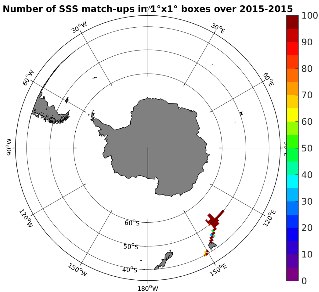
Figure 4: Number of SSS match-ups between TSG-GOSUD-Research-vessel SSS and the Aquarius-L4-IPRC-V4-WEEKLY SSS product for the Roaring Forties and Furious Fifties Pi-MEP region over 1^\circ \times 1^\circ boxes and for the full satellite product period.
