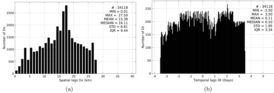
Figure 5: Histograms of the spatial (a) and temporal (b) lags between the time of the TSG-GOSUD-Research-vessel measurements and the date of the corresponding Aquarius-L4-IPRC-V4-WEEKLY SSS product.
