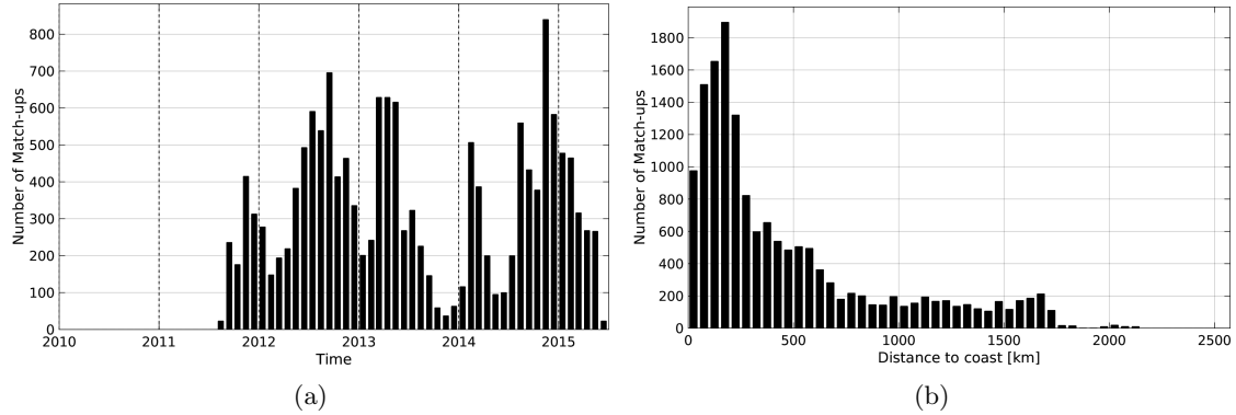
Figure 1: Number of match-ups between Sea mammals and Aquarius-L4-IPRC-V4-WEEKLY SSS as a function of time (a) and as function of the distance to coast (b) over the Roaring Forties and Furious Fifties Pi-MEP region and for the full satellite product period.
