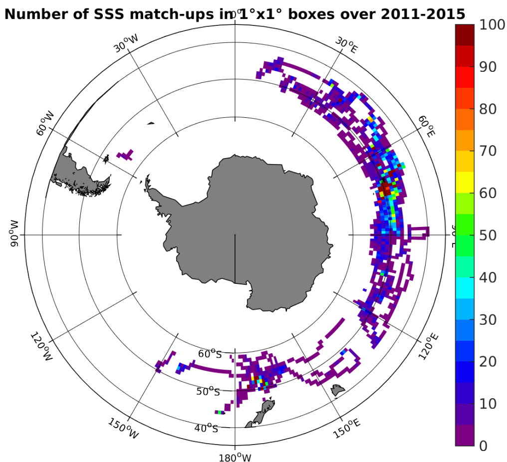
Figure 4: Number of SSS match-ups between Sea mammals SSS and the Aquarius-L4-IPRC-V4-WEEKLY SSS product for the Roaring Forties and Furious Fifties Pi-MEP region over 1°x1° boxes and for the full satellite product period.
