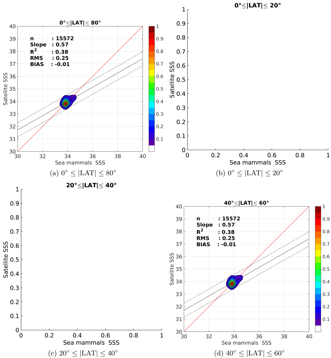
Figure 9: Contour maps of the concentration of Aquarius-L4-IPRC-V4-WEEKLY SSS (y-axis) versus Sea mammals SSS (x-axis) at match-up pairs for different latitude bands. For each plot, the red line shows x=y . The black thin and dashed lines indicate a linear fit through the data cloud and the \pm 95\% confidence levels, respectively. The number match-up pairs n , the slope and R^2 coefficient of the linear fit, the root mean square (RMS) and the mean bias between satellite and in situ data are indicated for each latitude band in each plots.
