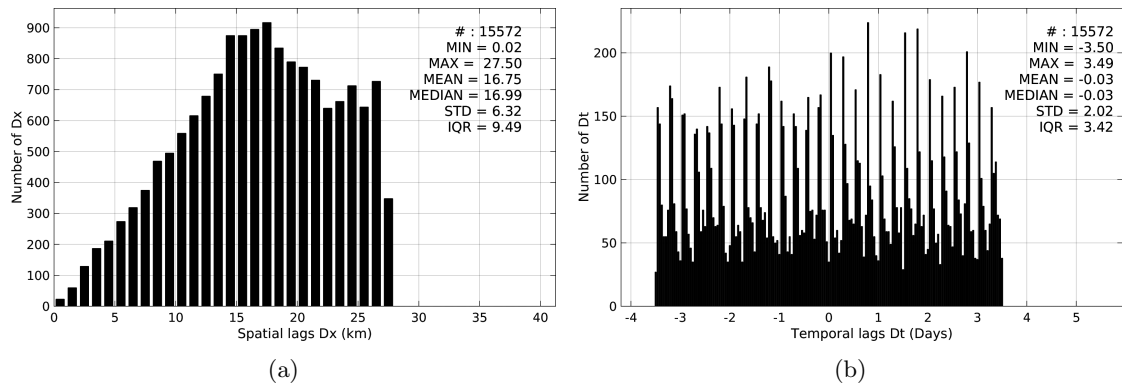
Figure 5: Histograms of the spatial (a) and temporal (b) lags between the time of the Sea mammals measurements and the date of the corresponding Aquarius-L4-IPRC-V4-WEEKLY SSS product.
