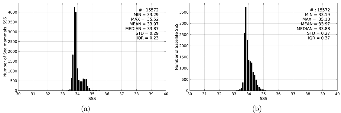
Figure 2: Histograms of SSS from Sea mammals (a) and Aquarius-L4-IPRC-V4-WEEKLY (b) considering all match-up pairs per bins of 0.1 over the Roaring Forties and Furious Fifties Pi-MEP region and for the full satellite product period.
