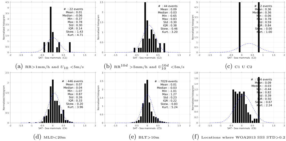
Figure 13: Normalized histogram of \Delta SSS (Aquarius-L4-IPRC-V4-WEEKLY - Sea mammals) for 6 different subdatasets corresponding to: RR > 1mm/h and U_{10} < 5 m/s (a), RR^{10d} > 5 mm/h and U_{10}^{10d} < 5 m/s (b), C1 U C2 (c), MLD < 20m (d), BLT > 10m (e), Locations where WOA2013 SSS STD > 0.2 (f).
