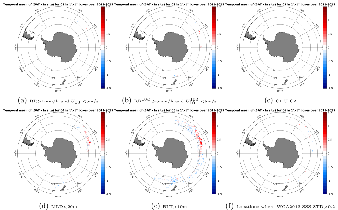
Figure 12: Temporal mean gridded over spatial boxes of size 1^\circ \times 1^\circ of \Delta SSS (Aquarius-L4-IPRC-V4-WEEKLY - Sea mammals) for 6 different subdatasets corresponding to: RR > 1\text{mm/h} and U_{10} < 5\text{m/s} (a), RR^{10d} > 5\text{mm/h} and U_{10}^{10d} < 5\text{m/s} (b), C1 U C2 (c), MLD < 20\text{m} (d), BLT > 10\text{m} (e), Locations where WOA2013 SSS STD > 0.2 (f).
