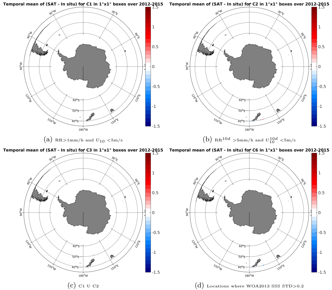
Figure 12: Temporal mean gridded over spatial boxes of size 1^\circ \times 1^\circ of \Delta SSS (Aquarius-L4-IPRC-V4-MONTHLY - TSG-LEGOS-DM) for 4 different subdatasets corresponding to: RR > 1 mm/h and U_{10} < 5 m/s (a), RR 10d > 5 mm/h and U_{10}^{10d} < 5 m/s (b), C1 U C2 (c), Locations where WOA2013 SSS STD > 0.2 (d).
