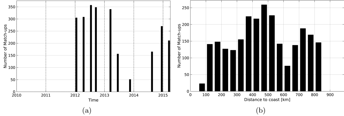
Figure 1: Number of match-ups between TSG-LEGOS-DM and Aquarius-L4-IPRC-V4-MONTHLY SSS as a function of time (a) and as function of the distance to coast (b) over the Roaring Forties and Furious Fifties Pi-MEP region and for the full satellite product period.
