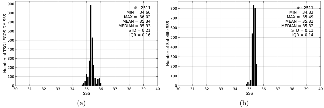
Figure 2: Histograms of SSS from TSG-LEGOS-DM (a) and Aquarius-L4-IPRC-V4-MONTHLY (b) considering all match-up pairs per bins of 0.1 over the Roaring Forties and Furious Fifties Pi-MEP region and for the full satellite product period.
