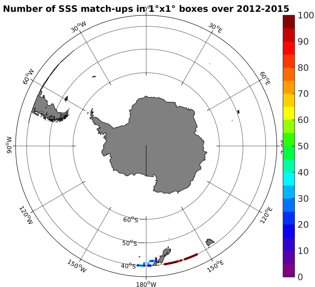
Figure 4: Number of SSS match-ups between TSG-LEGOS-DM SSS and the Aquarius-L4-IPRC-V4-MONTHLY SSS product for the Roaring Forties and Furious Fifties Pi-MEP region over 1^\circ \times 1^\circ boxes and for the full satellite product period.
