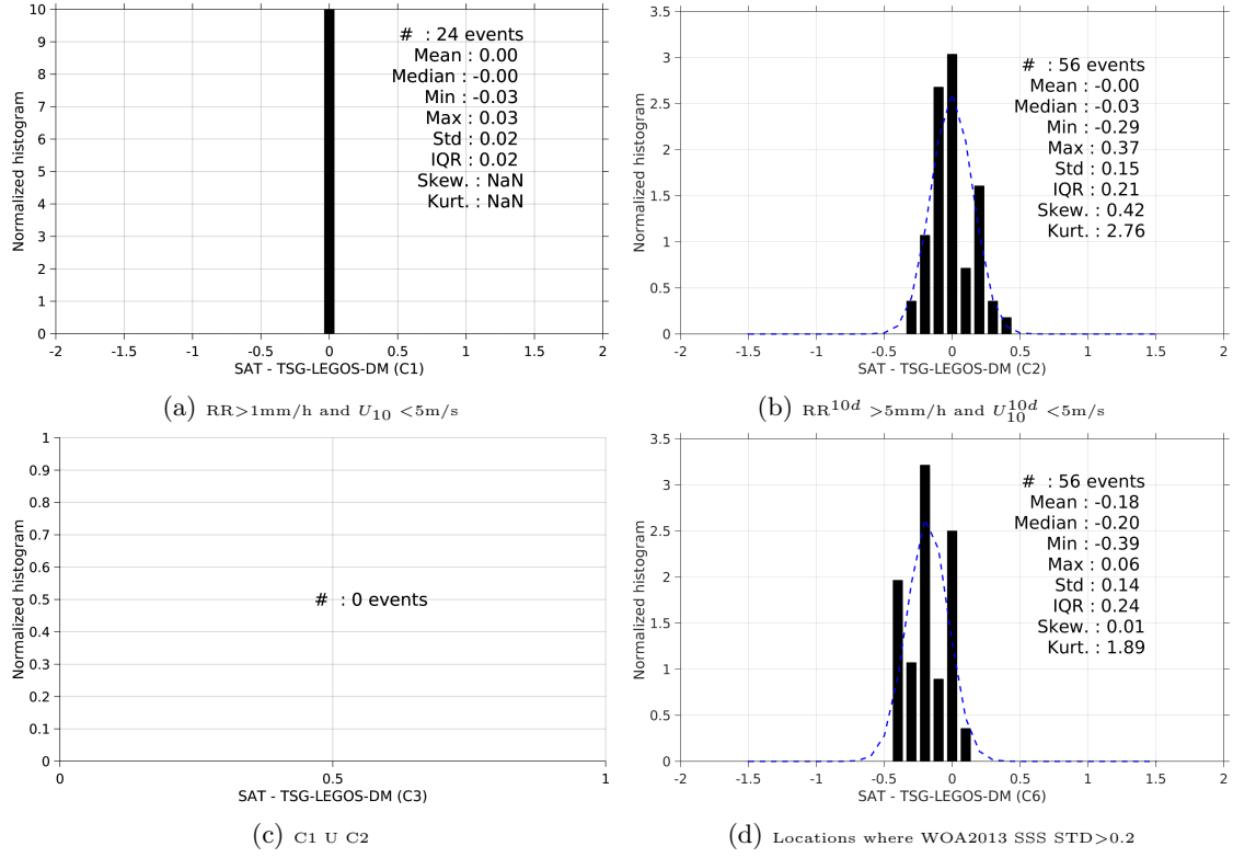
Figure 13: Normalized histogram of \Delta\text{SSS} (Aquarius-L4-IPRC-V4-MONTHLY - TSG-LEGOS-DM) for 6 different subdatasets corresponding to: RR > 1\text{mm/h} and U_{10} < 5\text{m/s} (a), RR^{10d} > 5\text{mm/h} and U_{10}^{10d} < 5\text{m/s} (b), C1 U C2 (c), Locations where WOA2013 SSS STD > 0.2 (d).
