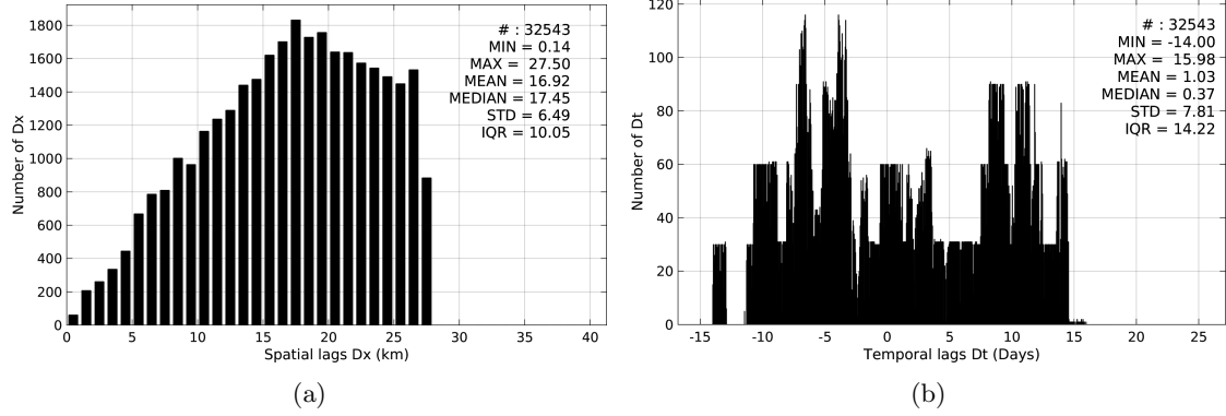
Figure 5: Histograms of the spatial (a) and temporal (b) lags between the time of the TSG-GOSUD-Sailing-ship measurements and the date of the corresponding Aquarius-L4-IPRC-V4-MONTHLY SSS product.
