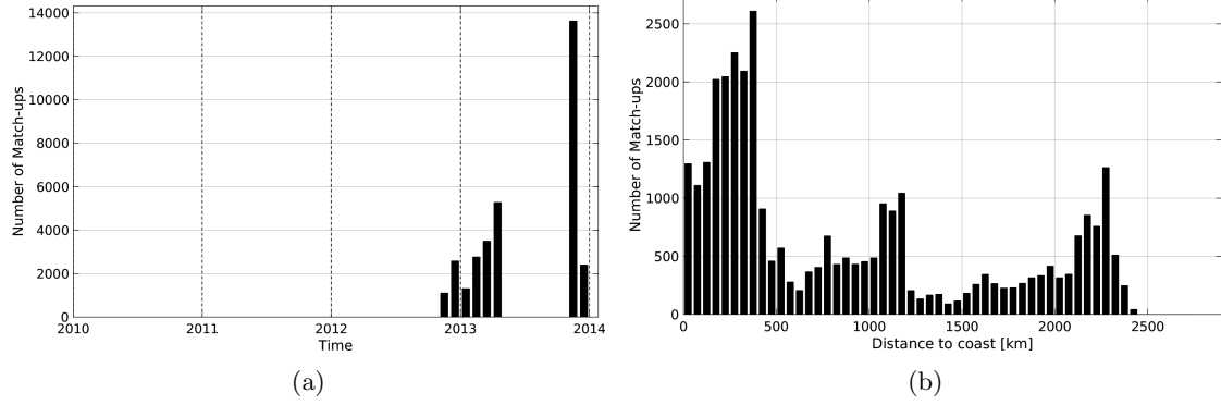
Figure 1: Number of match-ups between TSG-GOSUD-Sailing-ship and Aquarius-L4-IPRC-V4-MONTHLY SSS as a function of time (a) and as function of the distance to coast (b) over the Roaring Forties and Furious Fifties Pi-MEP region and for the full satellite product period.
