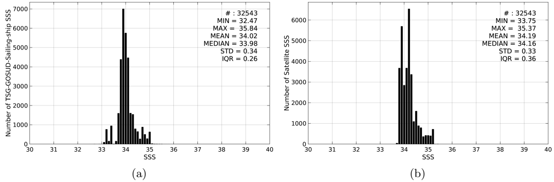
Figure 2: Histograms of SSS from TSG-GOSUD-Sailing-ship (a) and Aquarius-L4-IPRC-V4-MONTHLY (b) considering all match-up pairs per bins of 0.1 over the Roaring Forties and Furious Fifties Pi-MEP region and for the full satellite product period.
