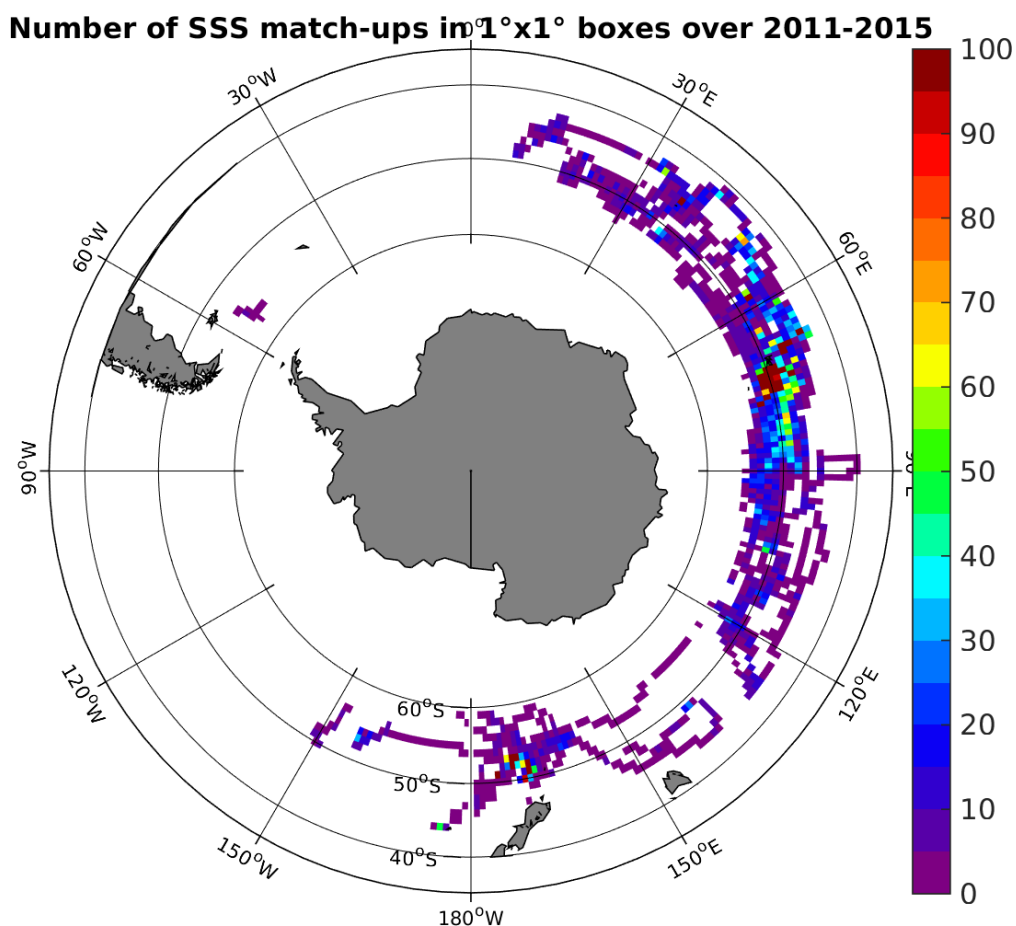
Figure 4: Number of SSS match-ups between Sea mammals SSS and the Aquarius-L4-IPRC-V4-MONTHLY SSS product for the Roaring Forties and Furious Fifties Pi-MEP region over 1^\circ \times 1^\circ boxes and for the full satellite product period.
