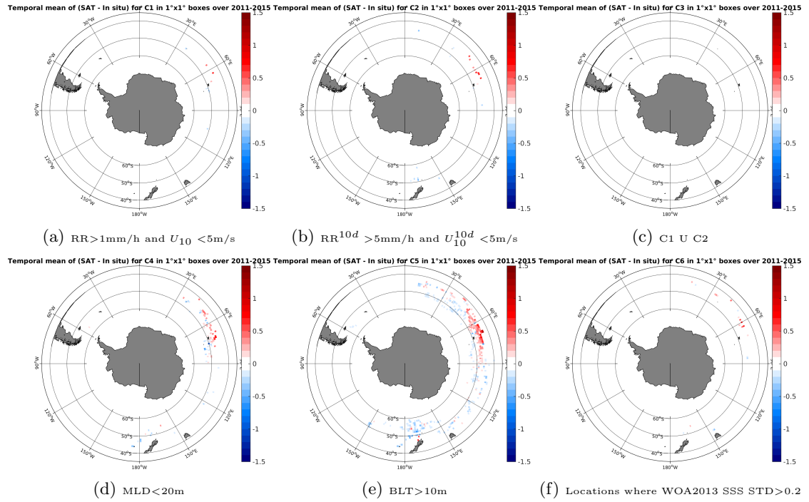
Figure 12: Temporal mean gridded over spatial boxes of size 1^\circ \times 1^\circ of \Delta SSS (Aquarius-L4-IPRC-V4-MONTHLY - Sea mammals) for 6 different subdatasets corresponding to: RR > 1\text{mm/h} and U_{10} < 5\text{m/s} (a), RR^{10d} > 5\text{mm/h} and U_{10}^{10d} < 5\text{m/s} (b), C1 U C2 (c), MLD < 20\text{m} (d), BLT > 10\text{m} (e), Locations where WOA2013 SSS STD > 0.2 (f).
