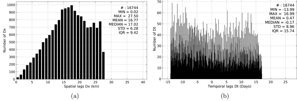
Figure 5: Histograms of the spatial (a) and temporal (b) lags between the time of the Sea mammals measurements and the date of the corresponding Aquarius-L4-IPRC-V4-MONTHLY SSS product.
