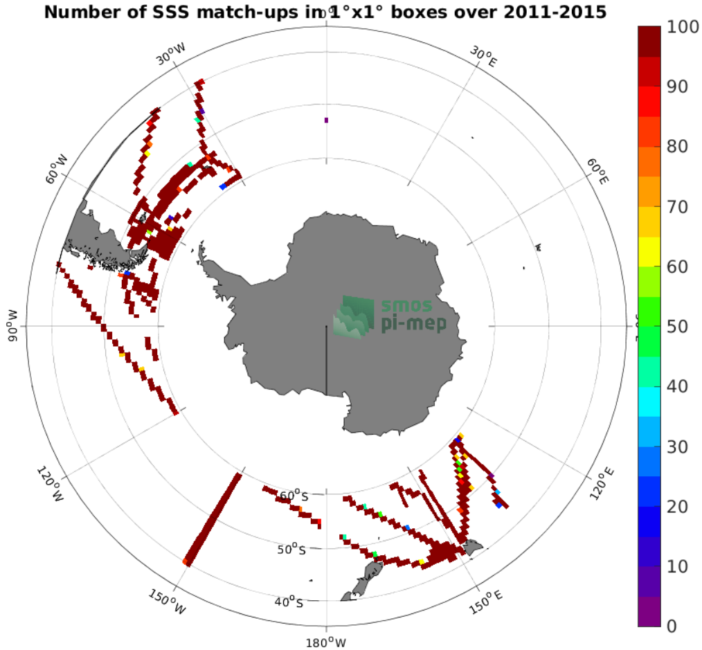
Figure 4: Number of SSS match-ups between TSG (SAMOS) SSS and the Aquarius SSS L3 OR v5 - 7-Day running (NASA-GSFC) SSS product for the Roaring Forties and Furious Fifties Pi-MEP region over 1^\circ \times 1^\circ boxes and for the full satellite product period.
