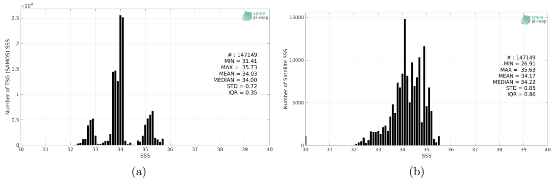
Figure 2: Histograms of SSS from TSG (SAMOS) (a) and Aquarius SSS L3 OR v5 - 7-Day running (NASA-GSFC) (b) considering all match-up pairs per bins of 0.1 over the Roaring Forties and Furious Fifties Pi-MEP region and for the full satellite product period.
