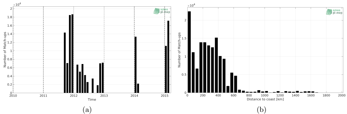
Figure 1: Number of match-ups between TSG (SAMOS) and Aquarius SSS L3 OR v5 - 7-Day running (NASA-GSFC) SSS as a function of time (a) and as function of the distance to coast (b) over the Roaring Forties and Furious Fifties Pi-MEP region and for the full satellite product period.
