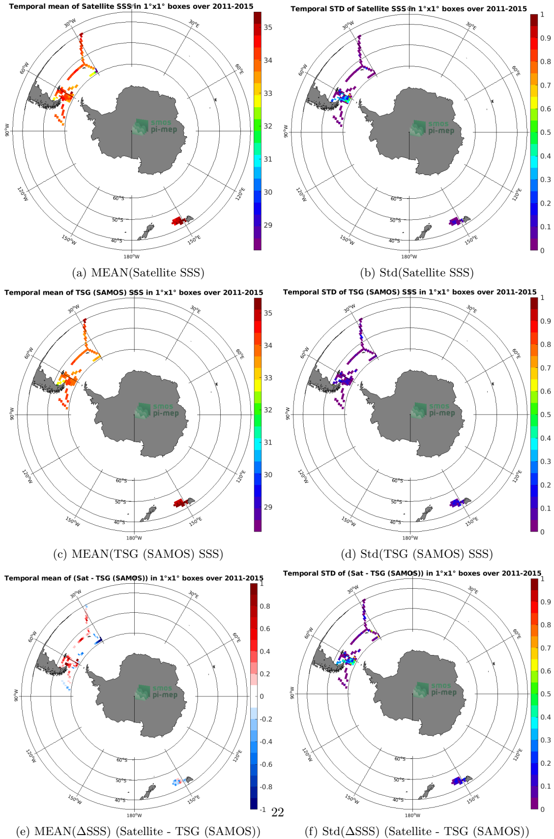
Figure 6: Temporal mean (left) and Std (right) of SSS from Aquarius SSS L3 OR v5 - 7-Day running (NASA-GSFC) (top), TSG (SAMOS) (middle), and of \Delta SSS (Satellite - TSG (SAMOS)). Only match-up pairs are used to generate these maps.
