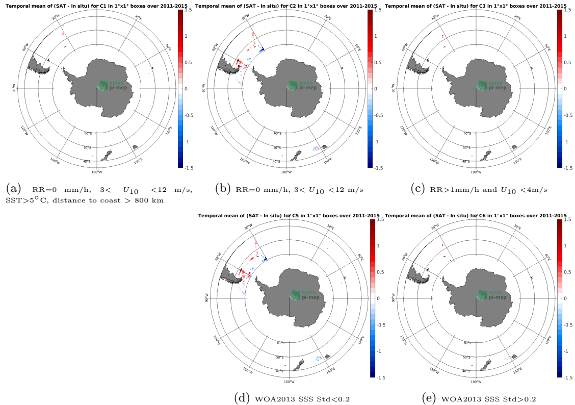
Figure 12: Temporal mean gridded over spatial boxes of size 1^{\circ}\times 1^{\circ} of \Delta\text{SSS} (Aquarius SSS L3 OR v5 - 7-Day running (NASA-GSFC) - TSG (SAMOS)) for 5 different subdatasets corresponding to:RR=0 mm/h, 3 < U_{10} < 12 m/s, SST >5^{\circ}\text{C} , distance to coast > 800 km (a), RR=0 mm/h, 3 < U_{10} < 12 m/s (b), RR >1 mm/h and U_{10} < 4 m/s (c), WOA2013 SSS Std <0.2 (d), WOA2013 SSS Std >0.2 (e).
