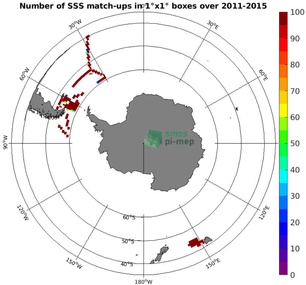
Figure 4: Number of SSS match-ups between TSG (SAMOS) SSS and the Aquarius SSS L3 OR v5 - 7-Day running (NASA-GSFC) SSS product for the Roaring Forties and Furious Fifties Pi-MEP region over 1^\circ \times 1^\circ boxes and for the full satellite product period.
