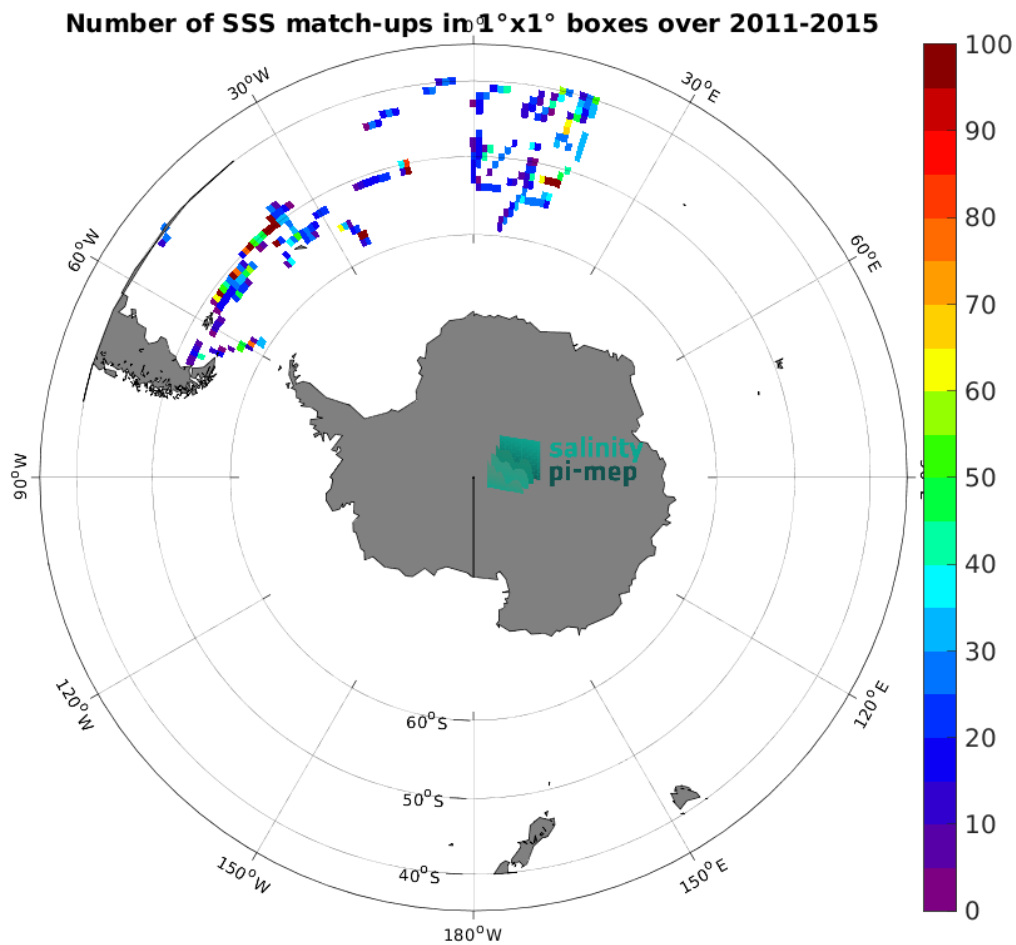
Figure 5: Number of SSS match-ups between TSG (Polarstern) SSS and the Aquarius SSS L3 OR v5 - 7-Day running (NASA-GSFC) SSS product for the Roaring Forties and Furious Fifties Pi-MEP region over 1^\circ \times 1^\circ boxes and for the full satellite product period.
