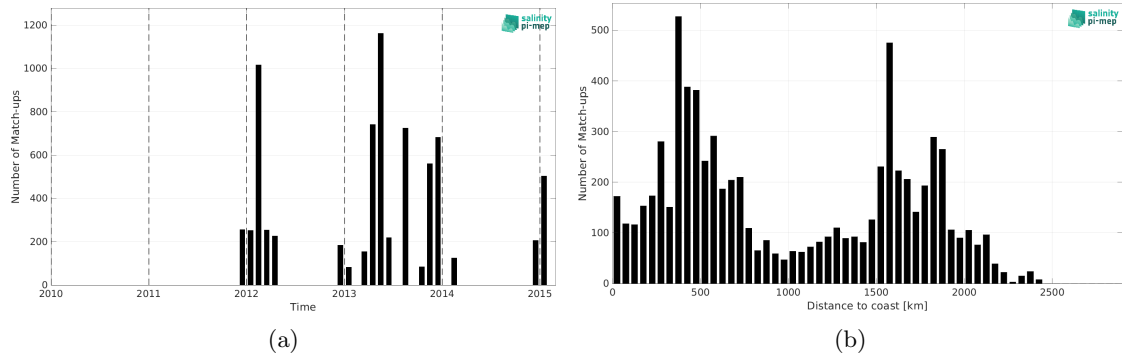
Figure 2: Number of match-ups between TSG (Polarstern) and Aquarius SSS L3 OR v5 - 7-Day running (NASA-GSFC) SSS as a function of time (a) and as function of the distance to coast (b) over the Roaring Forties and Furious Fifties Pi-MEP region and for the full satellite product period.
