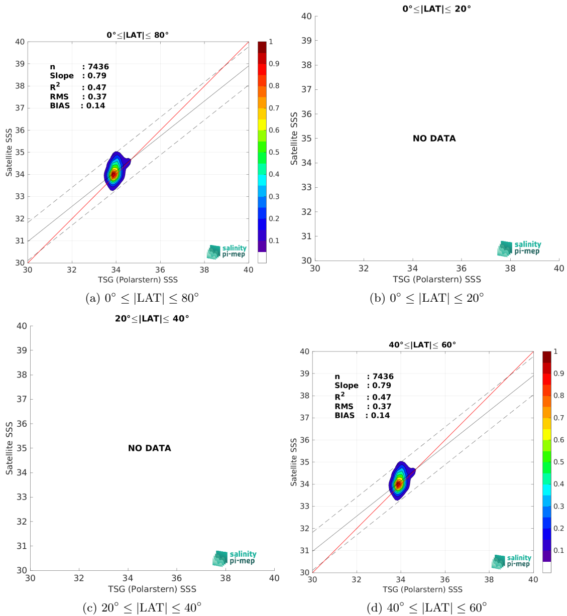
Figure 10: Contour maps of the concentration of Aquarius SSS L3 OR v5 - 7-Day running (NASA-GSFC) SSS (y-axis) versus TSG (Polarstern) SSS (x-axis) at match-up pairs for different latitude bands. For each plot, the red line shows x=y . The black thin and dashed lines indicate a linear fit through the data cloud and the \pm 95\% confidence levels, respectively. The number match-up pairs n , the slope and R^2 coefficient of the linear fit, the root mean square (RMS) and the mean bias between satellite and in situ data are indicated for each latitude band in each plots.
