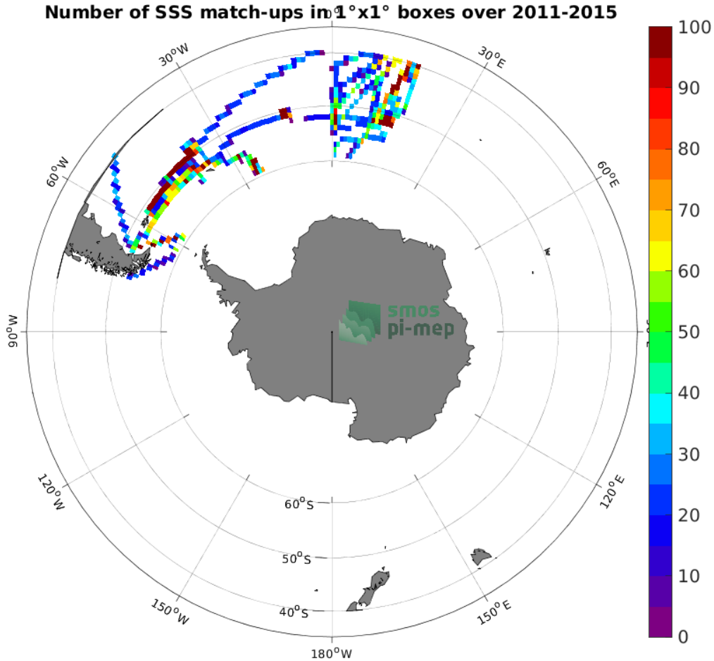
Figure 4: Number of SSS match-ups between TSG (Polarstern) SSS and the Aquarius SSS L3 OR v5 - 7-Day running (NASA-GSFC) SSS product for the Roaring Forties and Furious Fifties Pi-MEP region over 1^\circ \times 1^\circ boxes and for the full satellite product period.
