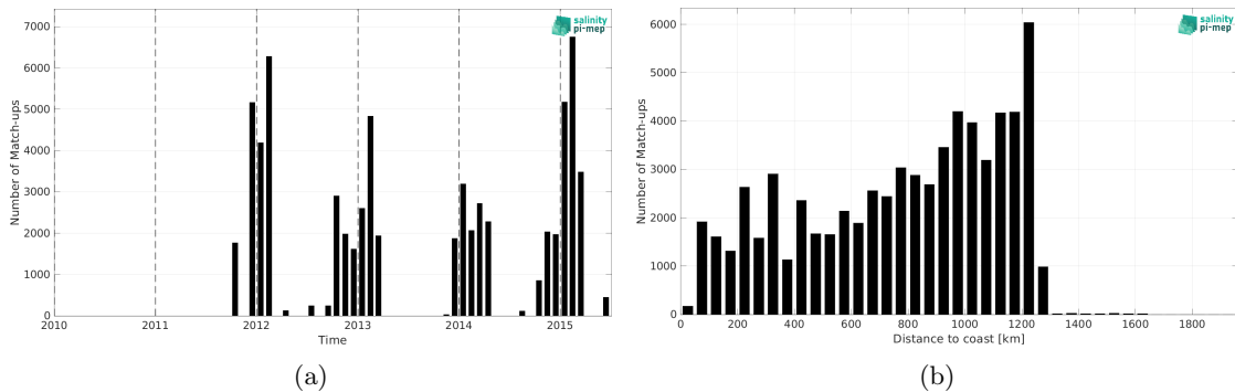
Figure 2: Number of match-ups between TSG (LEGOS-DM) and Aquarius SSS L3 OR v5 - 7-Day running (NASA-GSFC) SSS as a function of time (a) and as function of the distance to coast (b) over the Roaring Forties and Furious Fifties Pi-MEP region and for the full satellite product period.
