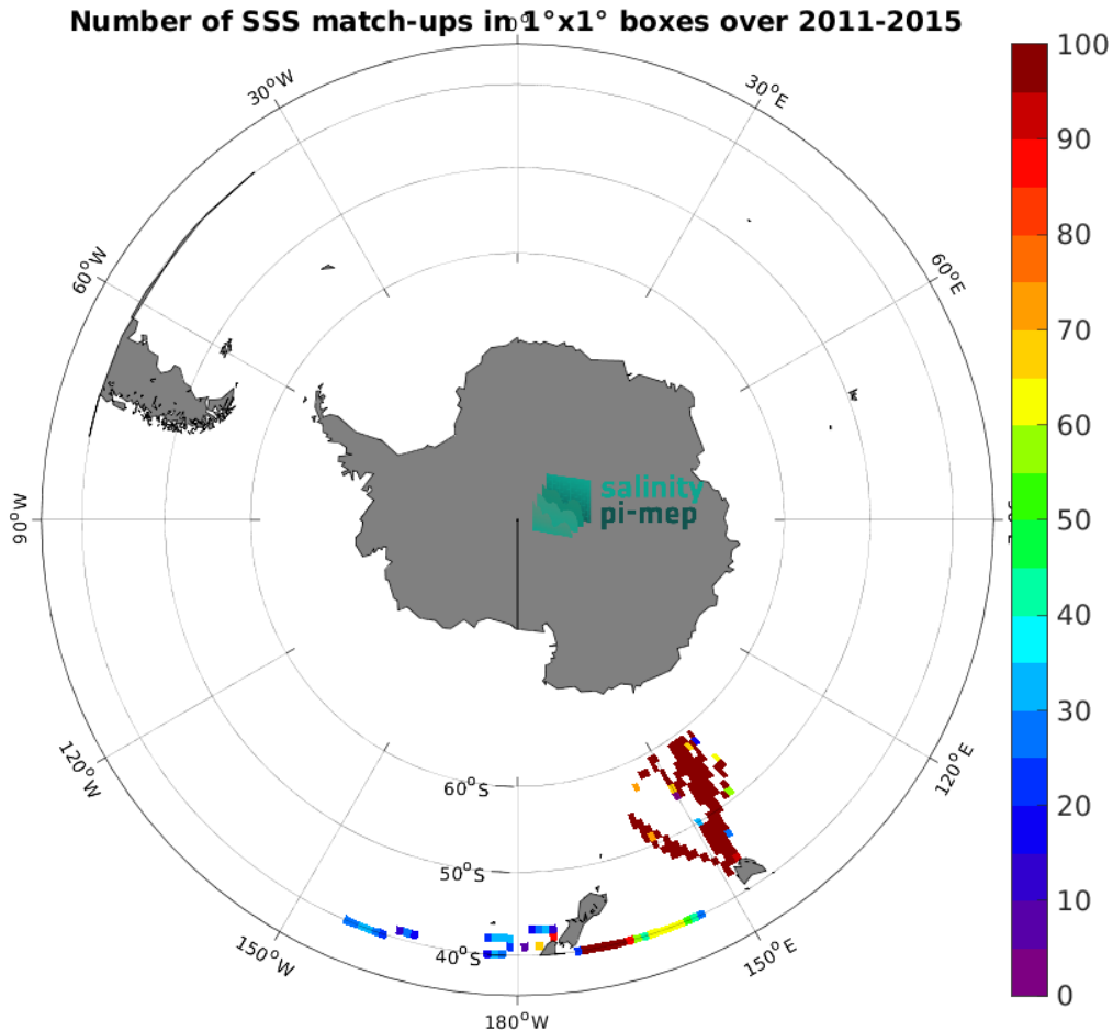
Figure 5: Number of SSS match-ups between TSG (LEGOS-DM) SSS and the Aquarius SSS L3 OR v5 - 7-Day running (NASA-GSFC) SSS product for the Roaring Forties and Furious Fifties Pi-MEP region over 1^\circ \times 1^\circ boxes and for the full satellite product period.
