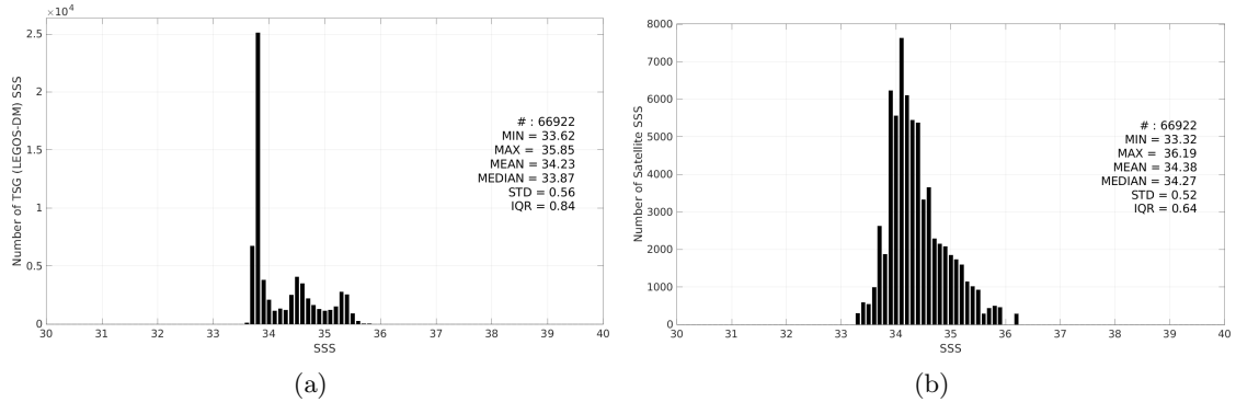
Figure 3: Histograms of SSS from TSG (LEGOS-DM) (a) and Aquarius SSS L3 OR v5 - 7-Day running (NASA-GSFC) (b) considering all match-up pairs per bins of 0.1 over the Roaring Forties and Furious Fifties Pi-MEP region and for the full satellite product period.
