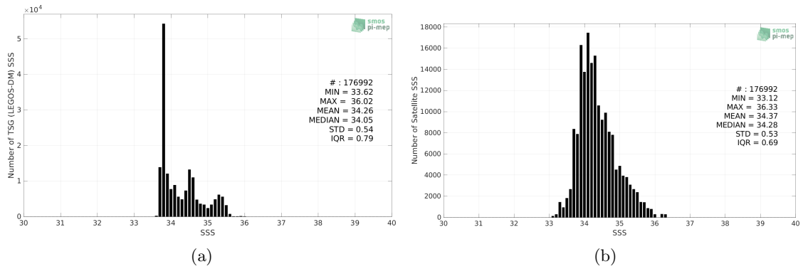
Figure 2: Histograms of SSS from TSG (LEGOS-DM) (a) and Aquarius SSS L3 OR v5 - 7-Day running (NASA-GSFC) (b) considering all match-up pairs per bins of 0.1 over the Roaring Forties and Furious Fifties Pi-MEP region and for the full satellite product period.
