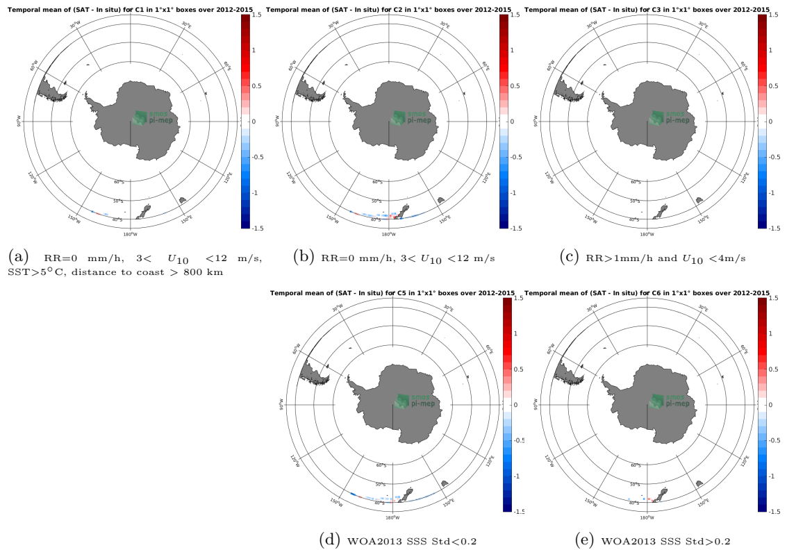
Figure 12: Temporal mean gridded over spatial boxes of size 1^{\circ}\times 1^{\circ} of \Delta\text{SSS} (Aquarius-L3-OR-V5-7DAY-RUNNING-1DEG - TSG-LEGOS-DM) for 5 different subdatasets corresponding to:RR=0 mm/h, 3 < U_{10} < 12 m/s, SST >5^{\circ}\text{C} , distance to coast > 800 km (a), RR=0 mm/h, 3 < U_{10} < 12 m/s (b), RR >1 mm/h and U_{10} < 4 m/s (c), WOA2013 SSS Std <0.2 (d), WOA2013 SSS Std >0.2 (e).
