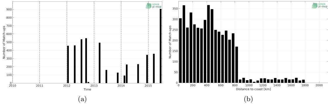
Figure 1: Number of match-ups between TSG-LEGOS-DM and Aquarius-L3-OR-V5-7DAY-RUNNING-1DEG SSS as a function of time (a) and as function of the distance to coast (b) over the Roaring Forties and Furious Fifties Pi-MEP region and for the full satellite product period.
