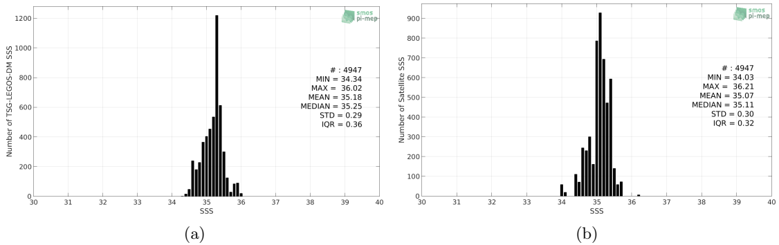
Figure 2: Histograms of SSS from TSG-LEGOS-DM (a) and Aquarius-L3-OR-V5-7DAY-RUNNING-1DEG (b) considering all match-up pairs per bins of 0.1 over the Roaring Forties and Furious Fifties Pi-MEP region and for the full satellite product period.
