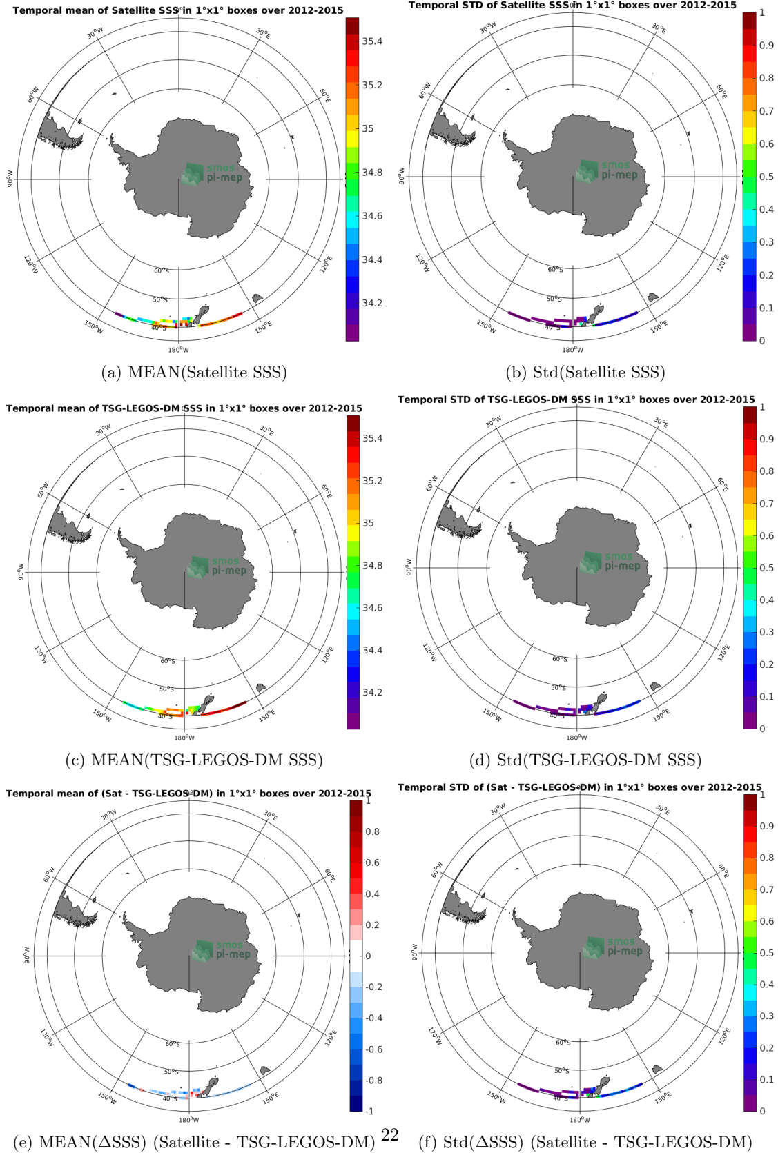
Figure 6: Temporal mean (left) and Std (right) of SSS from Aquarius-L3-OR-V5-7DAY-RUNNING-1DEG (top), TSG-LEGOS-DM (middle), and of \Delta SSS (Satellite - TSG-LEGOS-DM). Only match-up pairs are used to generate these maps.
