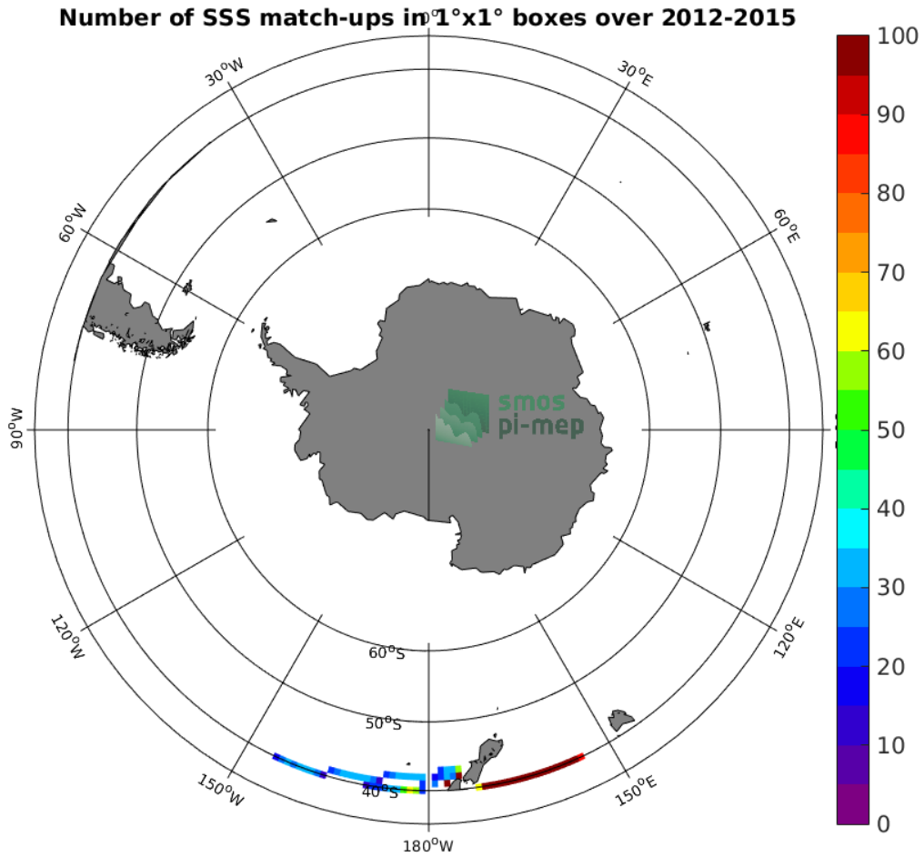
Figure 4: Number of SSS match-ups between TSG-LEGOS-DM SSS and the Aquarius-L3-OR-V5-7DAY-RUNNING-1DEG SSS product for the Roaring Forties and Furious Fifties Pi-MEP region over 1°x1° boxes and for the full satellite product period.
