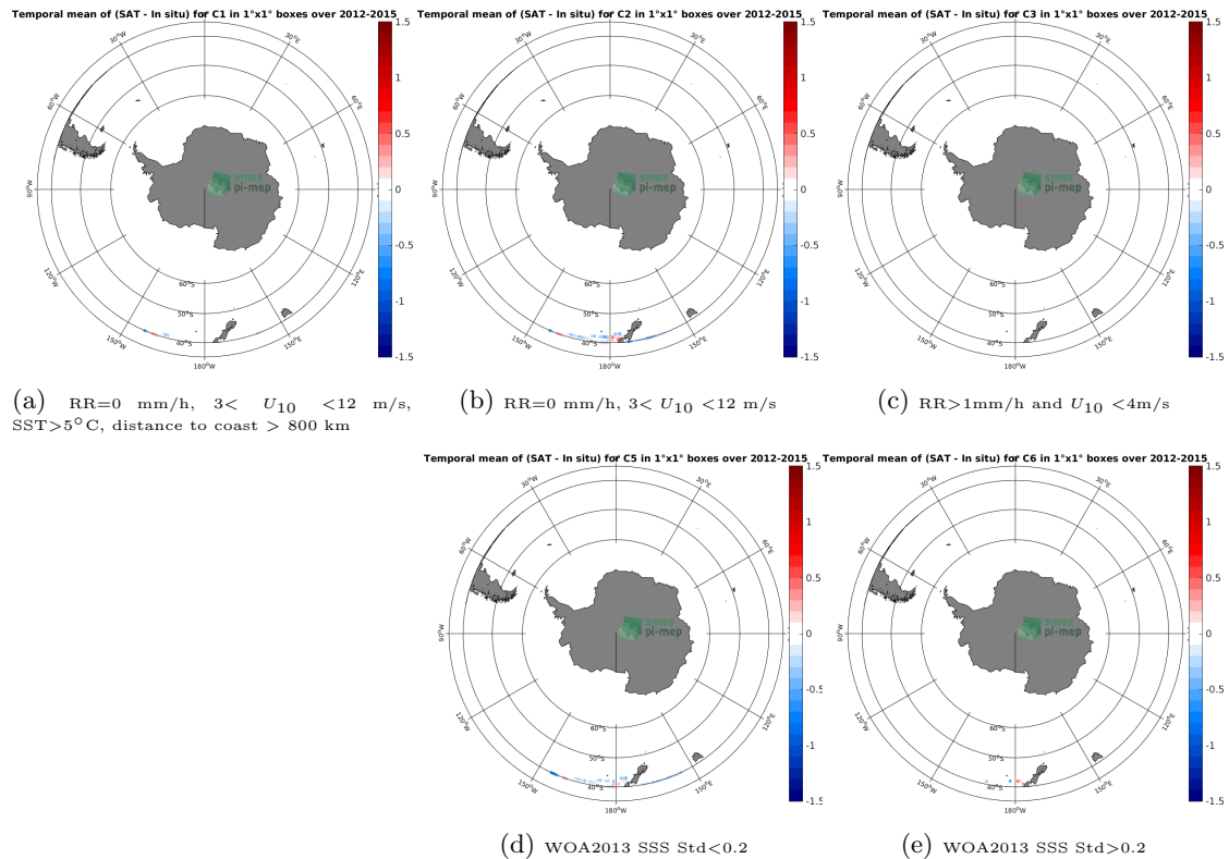
Figure 12: Temporal mean gridded over spatial boxes of size 1^\circ \times 1^\circ of \Delta SSS (Aquarius-L3-OR-V5-7DAY-RUNNING-1DEG - TSG-LEGOS-DM) for 5 different subdatasets corresponding to: RR=0 mm/h, 3 < U_{10} < 12 m/s, SST > 5^\circ\text{C} , distance to coast > 800 km (a), RR=0 mm/h, 3 < U_{10} < 12 m/s (b), RR > 1 mm/h and U_{10} < 4 m/s (c), WOA2013 SSS Std < 0.2 (d), WOA2013 SSS Std > 0.2 (e).
