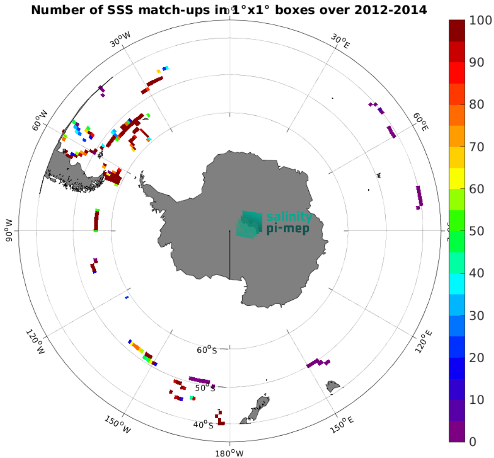
Figure 5: Number of SSS match-ups between TSG (GOSUD-Sailing-ship) SSS and the Aquarius SSS L3 OR v5 - 7-Day running (NASA-GSFC) SSS product for the Roaring Forties and Furious Fifties Pi-MEP region over 1^\circ \times 1^\circ boxes and for the full satellite product period.
