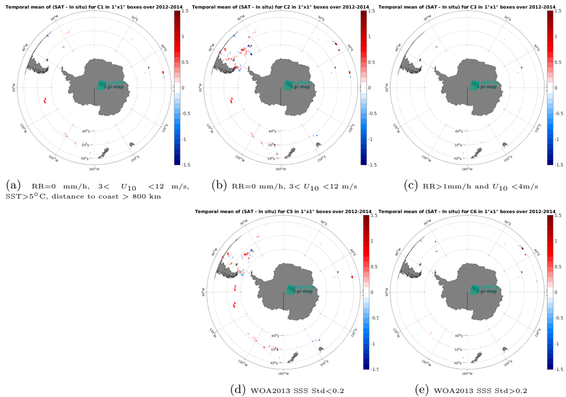
Figure 14: Temporal mean gridded over spatial boxes of size 1^\circ \times 1^\circ of \Delta SSS (Aquarius SSS L3 OR v5 - 7-Day running (NASA-GSFC) - TSG (GOSUD-Sailing-ship)) for 5 different subdatasets corresponding to: RR=0 mm/h, 3 < U_{10} < 12 m/s, SST > 5^\circ\text{C} , distance to coast > 800 km (a), RR=0 mm/h, 3 < U_{10} < 12 m/s (b), RR > 1 mm/h and U_{10} < 4 m/s (c), WOA2013 SSS Std < 0.2 (d), WOA2013 SSS Std > 0.2 (e).
