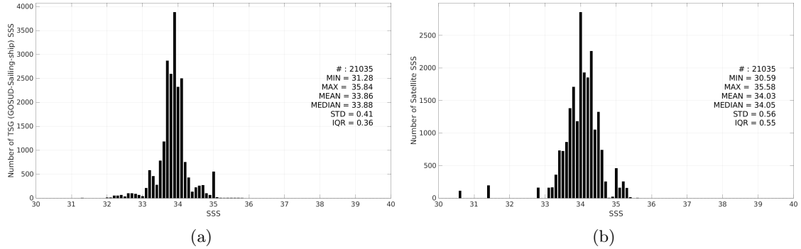
Figure 3: Histograms of SSS from TSG (GOSUD-Sailing-ship) (a) and Aquarius SSS L3 OR v5 - 7-Day running (NASA-GSFC) (b) considering all match-up pairs per bins of 0.1 over the Roaring Forties and Furious Fifties Pi-MEP region and for the full satellite product period.
