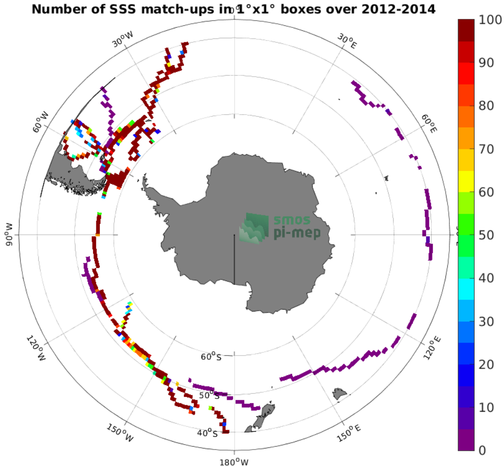
Figure 4: Number of SSS match-ups between TSG (GOSUD-Sailing-ship) SSS and the Aquarius SSS L3 OR v5 - 7-Day running (NASA-GSFC) SSS product for the Roaring Forties and Furious Fifties Pi-MEP region over 1^\circ \times 1^\circ boxes and for the full satellite product period.
