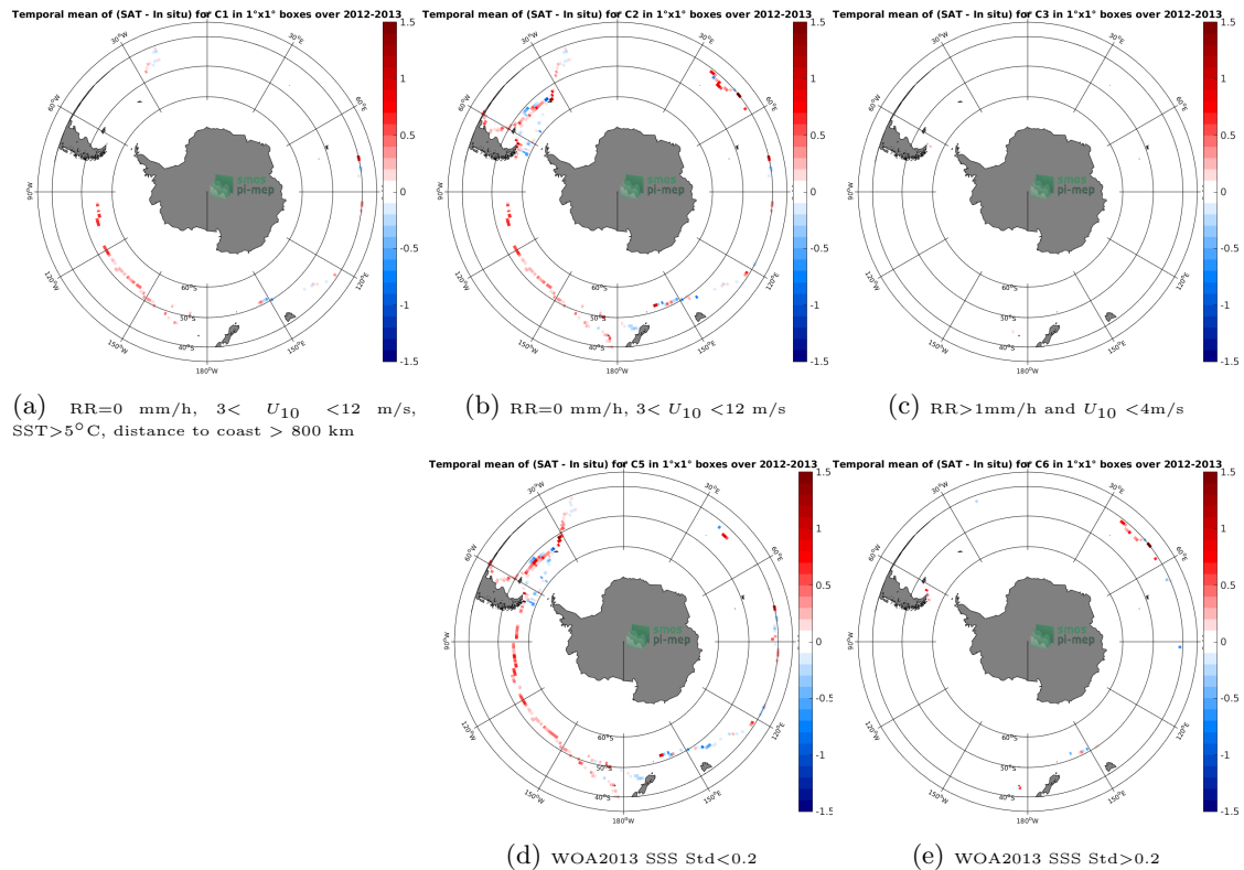
Figure 12: Temporal mean gridded over spatial boxes of size 1^\circ \times 1^\circ of \Delta SSS (Aquarius-L3-OR-V5-7DAY-RUNNING-1DEG - TSG-GOSUD-Sailing-ship) for 5 different subdatasets corresponding to:RR=0 mm/h, 3 < U_{10} < 12 m/s, SST >5^\circ C, distance to coast > 800 km (a), RR=0 mm/h, 3 < U_{10} < 12 m/s (b), RR >1 mm/h and U_{10} < 4 m/s (c), WOA2013 SSS Std <0.2 (d), WOA2013 SSS Std >0.2 (e).
