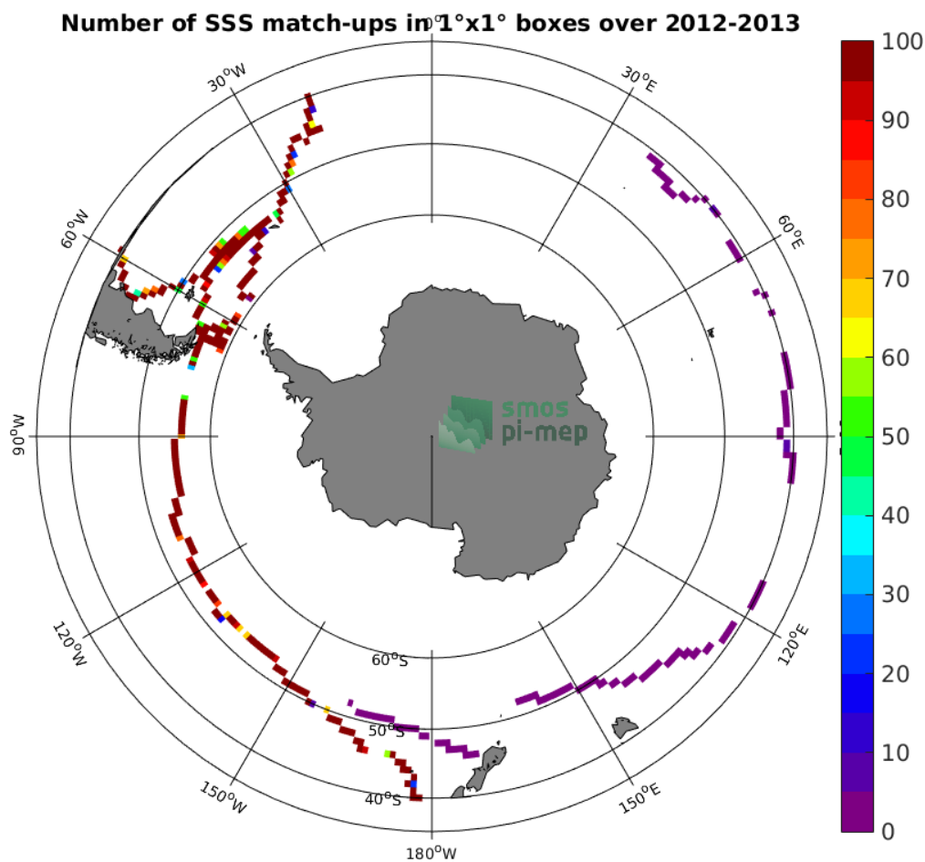
Figure 4: Number of SSS match-ups between TSG-GOSUD-Sailing-ship SSS and the Aquarius-L3-OR-V5-7DAY-RUNNING-1DEG SSS product for the Roaring Forties and Furious Fifties Pi-MEP region over 1°x1° boxes and for the full satellite product period.
