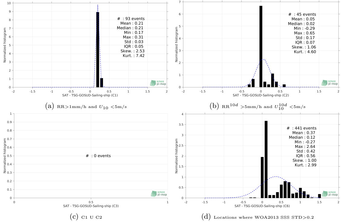
Figure 13: Normalized histogram of \Delta\text{SSS} (Aquarius-L3-OR-V5-7DAY-RUNNING-1DEG - TSG-GOSUD-Sailing-ship) for 6 different subdatasets corresponding to: RR > 1mm/h and U_{10} < 5\text{m/s} (a), RR^{10d} > 5\text{mm/h} and U_{10}^{10d} < 5\text{m/s} (b), C1 U C2 (c), Locations where WOA2013 SSS STD > 0.2 (d).
