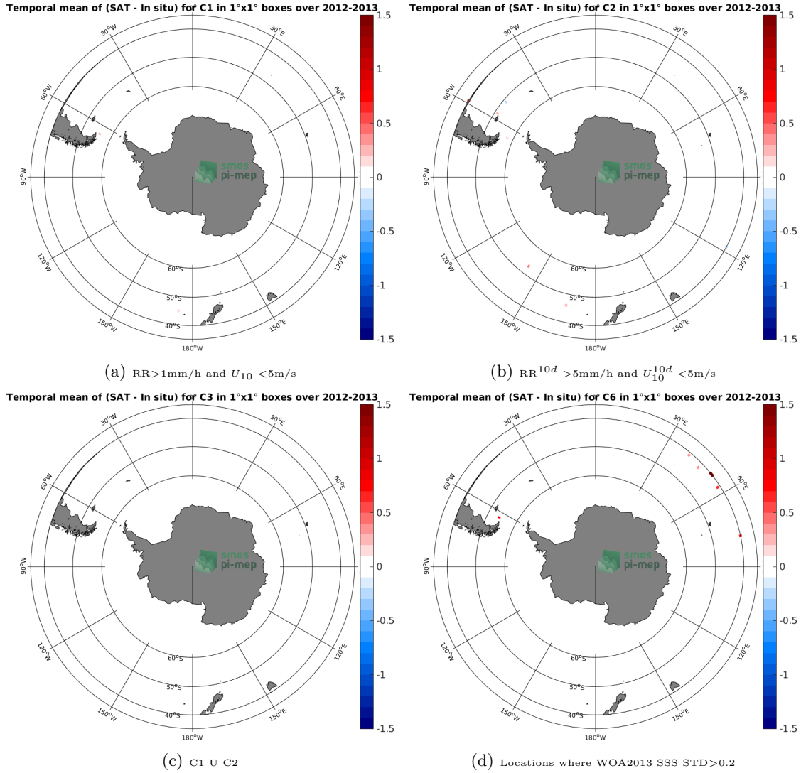
Figure 12: Temporal mean gridded over spatial boxes of size 1^\circ \times 1^\circ of \Delta SSS (Aquarius-L3-OR-V5-7DAY-RUNNING-1DEG - TSG-GOSUD-Sailing-ship) for 4 different subdatasets corresponding to: RR > 1\text{mm/h} and U_{10} < 5\text{m/s} (a), RR^{10d} > 5\text{mm/h} and U_{10}^{10d} < 5\text{m/s} (b), C1 U C2 (c), Locations where WOA2013 SSS STD > 0.2 (d).
