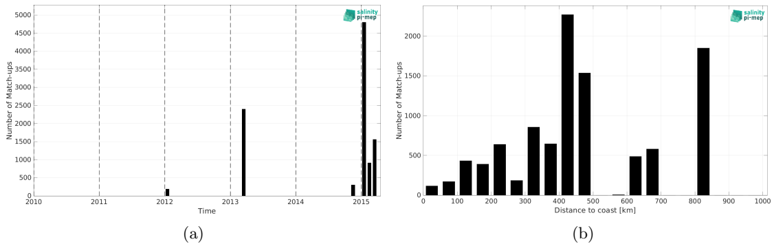
Figure 2: Number of match-ups between TSG (CSIC-UTM) and Aquarius SSS L3 OR v5 - 7-Day running (NASA-GSFC) SSS as a function of time (a) and as function of the distance to coast (b) over the Roaring Forties and Furious Fifties Pi-MEP region and for the full satellite product period.
