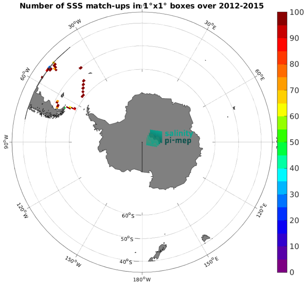
Figure 5: Number of SSS match-ups between TSG (CSIC-UTM) SSS and the Aquarius SSS L3 OR v5 - 7-Day running (NASA-GSFC) SSS product for the Roaring Forties and Furious Fifties Pi-MEP region over 1^\circ \times 1^\circ boxes and for the full satellite product period.
