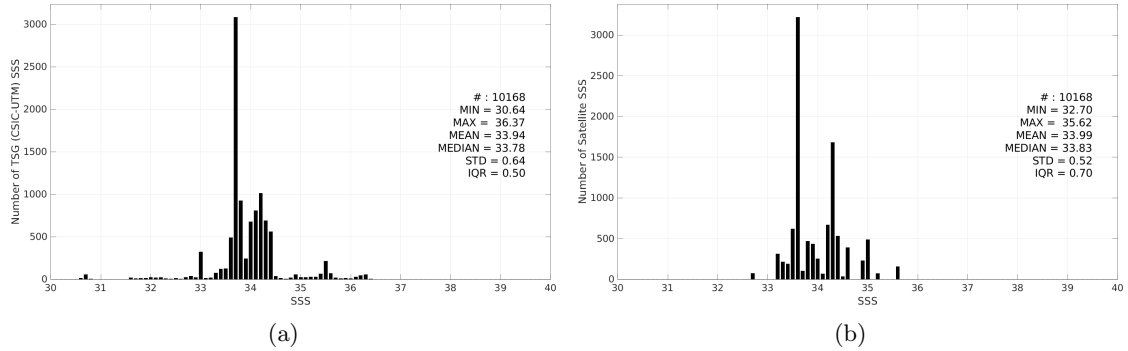
Figure 3: Histograms of SSS from TSG (CSIC-UTM) (a) and Aquarius SSS L3 OR v5 - 7-Day running (NASA-GSFC) (b) considering all match-up pairs per bins of 0.1 over the Roaring Forties and Furious Fifties Pi-MEP region and for the full satellite product period.
