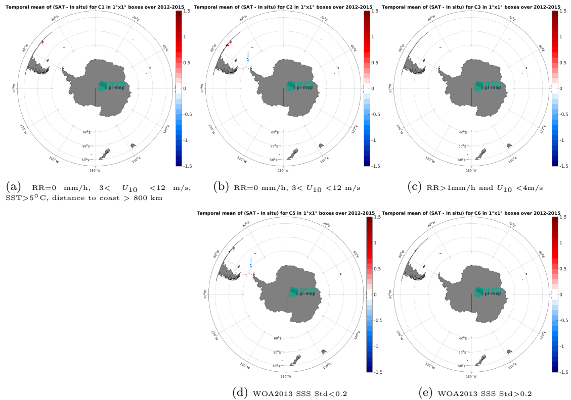
Figure 14: Temporal mean gridded over spatial boxes of size 1^\circ \times 1^\circ of \Delta SSS (Aquarius SSS L3 OR v5 - 7-Day running (NASA-GSFC) - TSG (CSIC-UTM)) for 5 different subdatasets corresponding to:RR=0 mm/h, 3 < U_{10} < 12 m/s, SST>5°C, distance to coast > 800 km (a), RR=0 mm/h, 3 < U_{10} < 12 m/s (b), RR>1mm/h and U_{10} < 4 m/s (c), WOA2013 SSS Std<0.2 (d), WOA2013 SSS Std>0.2 (e).
