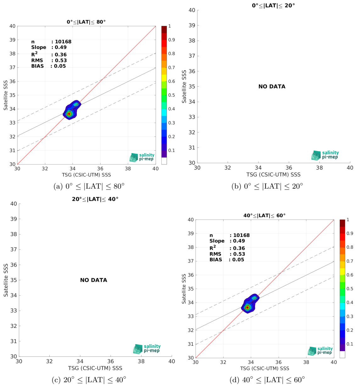
Figure 10: Contour maps of the concentration of Aquarius SSS L3 OR v5 - 7-Day running (NASA-GSFC) SSS (y-axis) versus TSG (CSIC-UTM) SSS (x-axis) at match-up pairs for different latitude bands. For each plot, the red line shows x=y . The black thin and dashed lines indicate a linear fit through the data cloud and the \pm 95\% confidence levels, respectively. The number match-up pairs n , the slope and R^2 coefficient of the linear fit, the root mean square (RMS) and the mean bias between satellite and in situ data are indicated for each latitude band in each plots.
