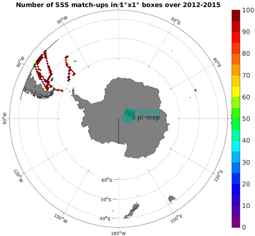
Figure 4: Number of SSS match-ups between TSG (CSIC-UTM) SSS and the Aquarius SSS L3 OR v5 - 7-Day running (NASA-GSFC) SSS product for the Roaring Forties and Furious Fifties Pi-MEP region over 1^\circ \times 1^\circ boxes and for the full satellite product period.
