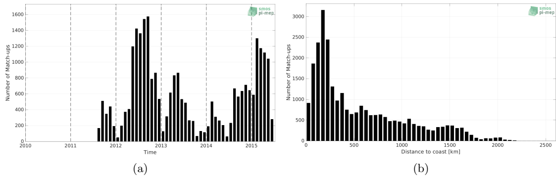
Figure 1: Number of match-ups between Marine mammals and Aquarius SSS L3 OR v5 - 7-Day running (NASA-GSFC) SSS as a function of time (a) and as function of the distance to coast (b) over the Roaring Forties and Furious Fifties Pi-MEP region and for the full satellite product period.
