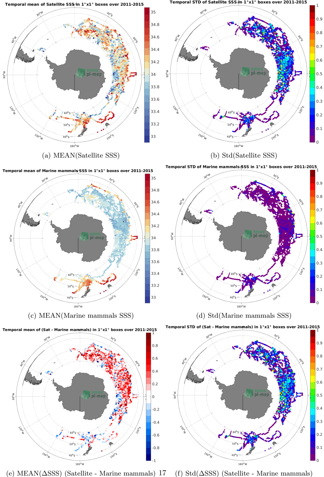
Figure 6: Temporal mean (left) and Std (right) of SSS from Aquarius SSS L3 OR v5 - 7-Day running (NASA-GSFC) (top), Marine mammals (middle), and of \Delta SSS (Satellite - Marine mammals). Only match-up pairs are used to generate these maps.
