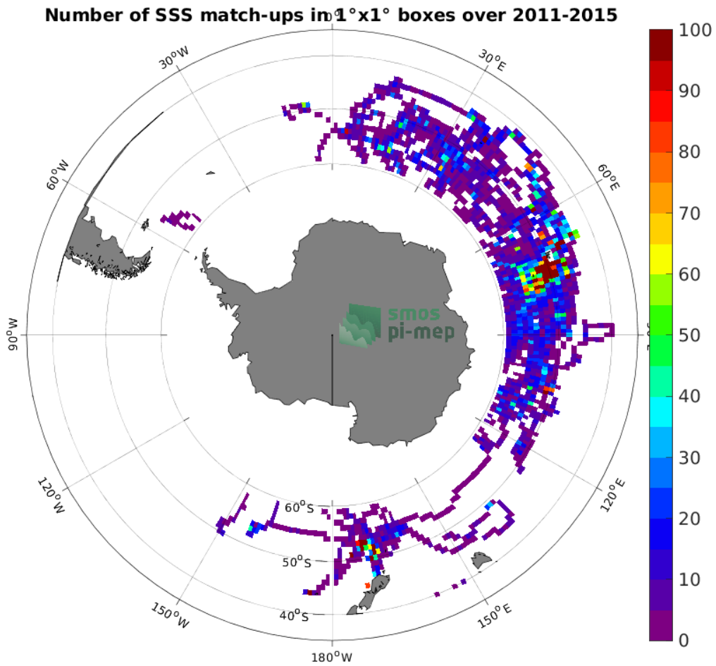
Figure 4: Number of SSS match-ups between Marine mammals SSS and the Aquarius SSS L3 OR v5 - 7-Day running (NASA-GSFC) SSS product for the Roaring Forties and Furious Fifties Pi-MEP region over 1^\circ \times 1^\circ boxes and for the full satellite product period.
