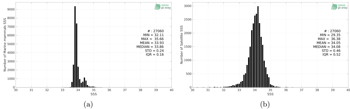
Figure 2: Histograms of SSS from Marine mammals (a) and Aquarius SSS L3 OR v5 - 7-Day running (NASA-GSFC) (b) considering all match-up pairs per bins of 0.1 over the Roaring Forties and Furious Fifties Pi-MEP region and for the full satellite product period.
