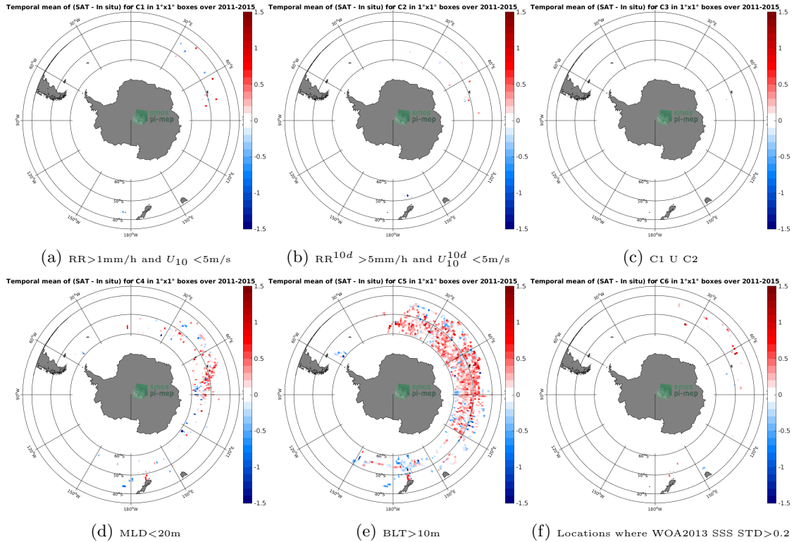
Figure 12: Temporal mean gridded over spatial boxes of size 1^\circ \times 1^\circ of \Delta SSS (Aquarius-L3-OR-V5-7DAY-RUNNING-1DEG - Sea mammals) for 6 different subdatasets corresponding to: RR > 1\text{mm/h} and U_{10} < 5\text{m/s} (a), RR^{10d} > 5\text{mm/h} and U_{10}^{10d} < 5\text{m/s} (b), C1 U C2 (c), MLD < 20\text{m} (d), BLT > 10\text{m} (e), Locations where WOA2013 SSS STD > 0.2 (f).
