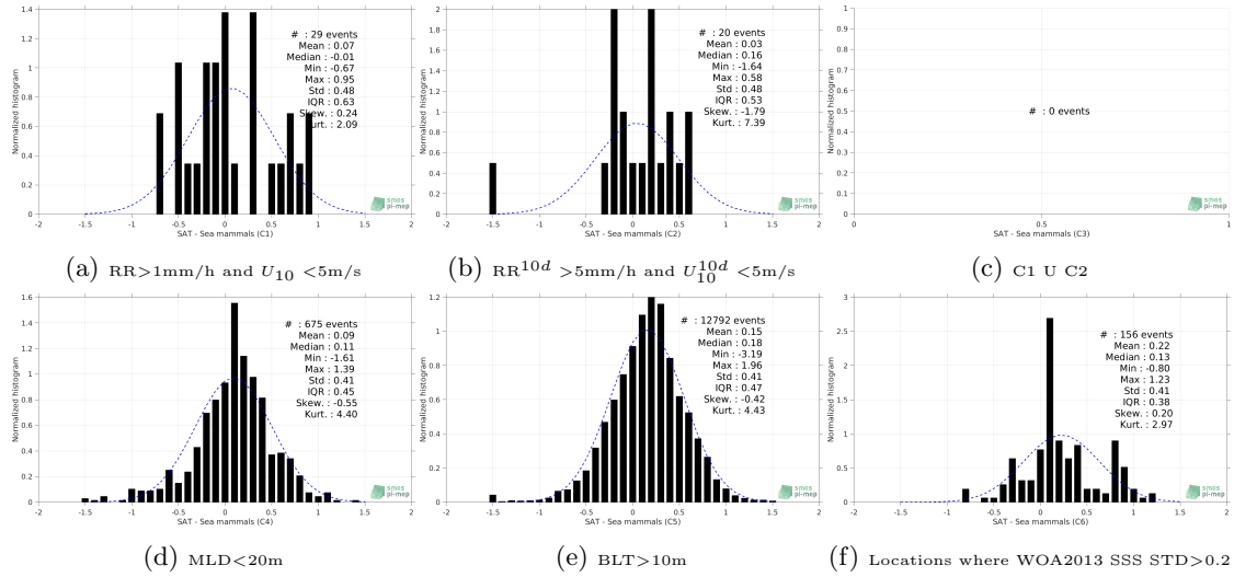
Figure 13: Normalized histogram of \Delta SSS (Aquarius-L3-OR-V5-7DAY-RUNNING-1DEG - Sea mammals) for 6 different subdatasets corresponding to: RR > 1\text{mm/h} and U_{10} < 5\text{m/s} (a), RR^{10d} > 5\text{mm/h} and U_{10}^{10d} < 5\text{m/s} (b), C1 U C2 (c), MLD < 20\text{m} (d), BLT > 10\text{m} (e), Locations where WOA2013 SSS STD > 0.2 (f).
