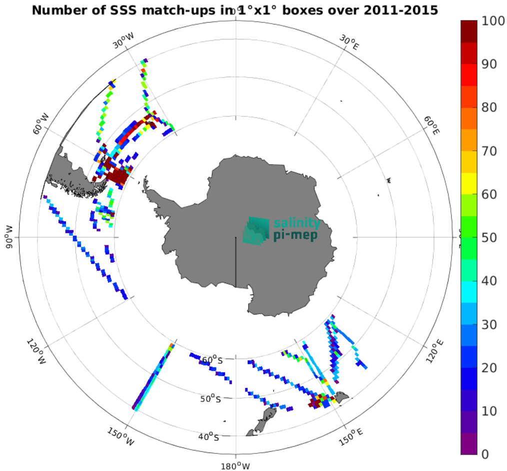
Figure 5: Number of SSS match-ups between TSG (SAMOS) SSS and the Aquarius SSS L3 OR v5 - 7-Day running - Rain mask (NASA-GSFC) SSS product for the Roaring Forties and Furious Fifties Pi-MEP region over 1^\circ \times 1^\circ boxes and for the full satellite product period.
