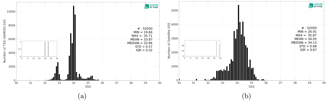
Figure 3: Histograms of SSS from TSG (SAMOS) (a) and Aquarius SSS L3 OR v5 - 7-Day running - Rain mask (NASA-GSFC) (b) considering all match-up pairs per bins of 0.1 over the Roaring Forties and Furious Fifties Pi-MEP region and for the full satellite product period.
