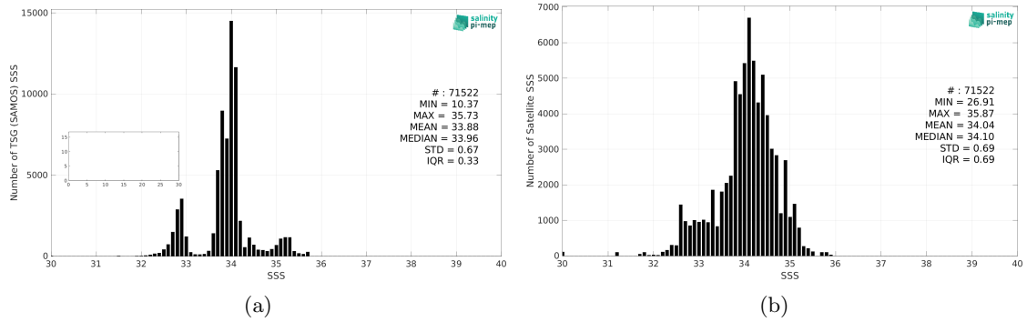
Figure 2: Histograms of SSS from TSG (SAMOS) (a) and Aquarius SSS L3 OR v5 - 7-Day running - Rain mask (NASA-GSFC) (b) considering all match-up pairs per bins of 0.1 over the Roaring Forties and Furious Fifties Pi-MEP region and for the full satellite product period.
