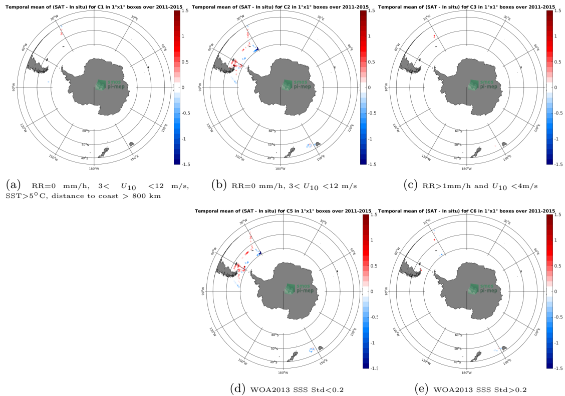
Figure 12: Temporal mean gridded over spatial boxes of size 1^{\circ}\times 1^{\circ} of \Delta\text{SSS} (Aquarius-L3-OR-V5-7DAY-RUNNING-RAIN-MASK-1DEG - TSG-SAMOS) for 5 different subdatasets corresponding to: \text{RR}=0 mm/h, 3 < U_{10} < 12 m/s, \text{SST}>5^{\circ}\text{C} , distance to coast > 800 km (a), \text{RR}=0 mm/h, 3 < U_{10} < 12 m/s (b), \text{RR}>1 mm/h and U_{10} < 4 m/s (c), WOA2013 SSS Std < 0.2 (d), WOA2013 SSS Std > 0.2 (e).
