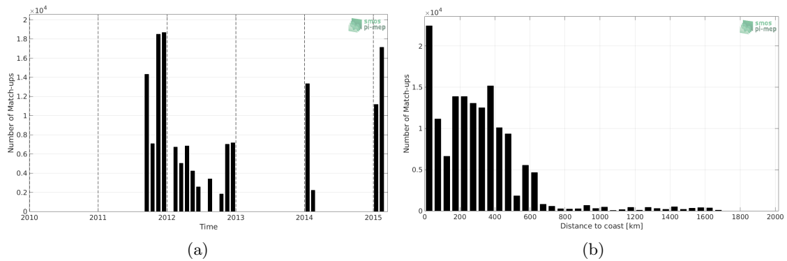
Figure 1: Number of match-ups between TSG-SAMOS and Aquarius-L3-OR-V5-7DAY-RUNNING-RAIN-MASK-1DEG SSS as a function of time (a) and as function of the distance to coast (b) over the Roaring Forties and Furious Fifties Pi-MEP region and for the full satellite product period.
