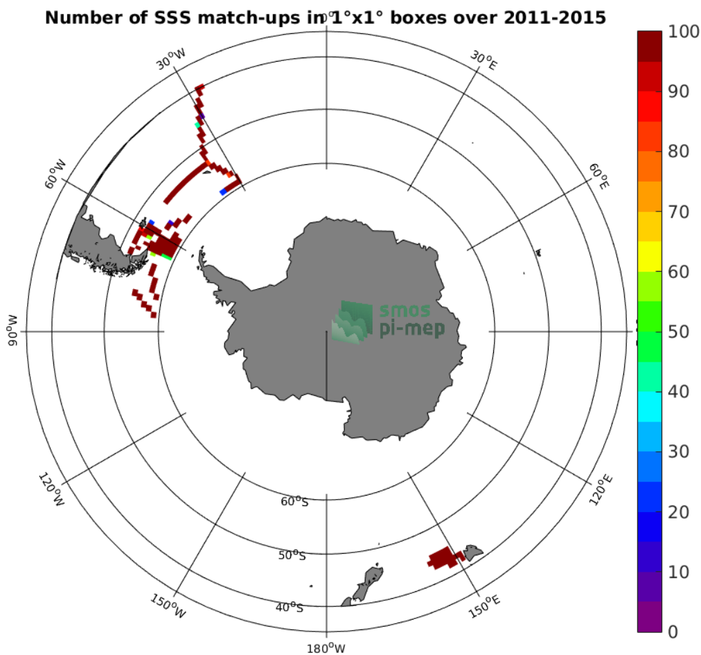
Figure 4: Number of SSS match-ups between TSG-SAMOS SSS and the Aquarius-L3-OR-V5-7DAY-RUNNING-RAIN-MASK-1DEG SSS product for the Roaring Forties and Furious Fifties Pi-MEP region over 1°x1° boxes and for the full satellite product period.
