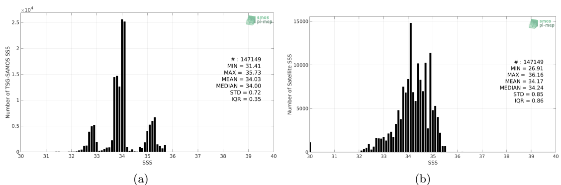
Figure 2: Histograms of SSS from TSG-SAMOS (a) and Aquarius-L3-OR-V5-7DAY-RUNNING-RAIN-MASK-1DEG (b) considering all match-up pairs per bins of 0.1 over the Roaring Forties and Furious Fifties Pi-MEP region and for the full satellite product period.
