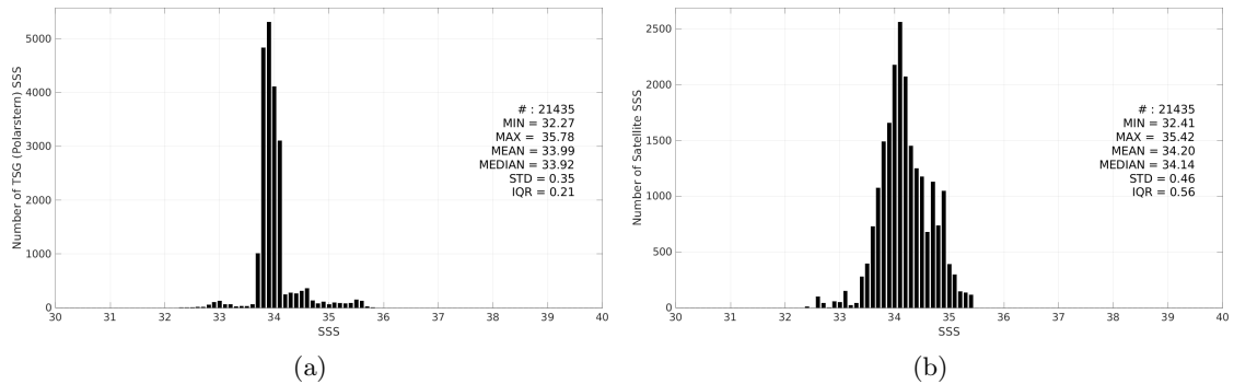
Figure 3: Histograms of SSS from TSG (Polarstern) (a) and Aquarius SSS L3 OR v5 - 7-Day running - Rain mask (NASA-GSFC) (b) considering all match-up pairs per bins of 0.1 over the Roaring Forties and Furious Fifties Pi-MEP region and for the full satellite product period.
