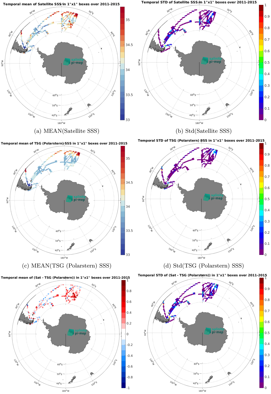
Figure 7: Temporal mean (left) and Std (right) of SSS from Aquarius SSS L3 OR v5 - 7-Day running - Rain mask (NASA-GSFC) (top), TSG (Polarstern) (middle), and of \Delta SSS (Satellite - TSG (Polarstern)). Only match-up pairs are used to generate these maps.
