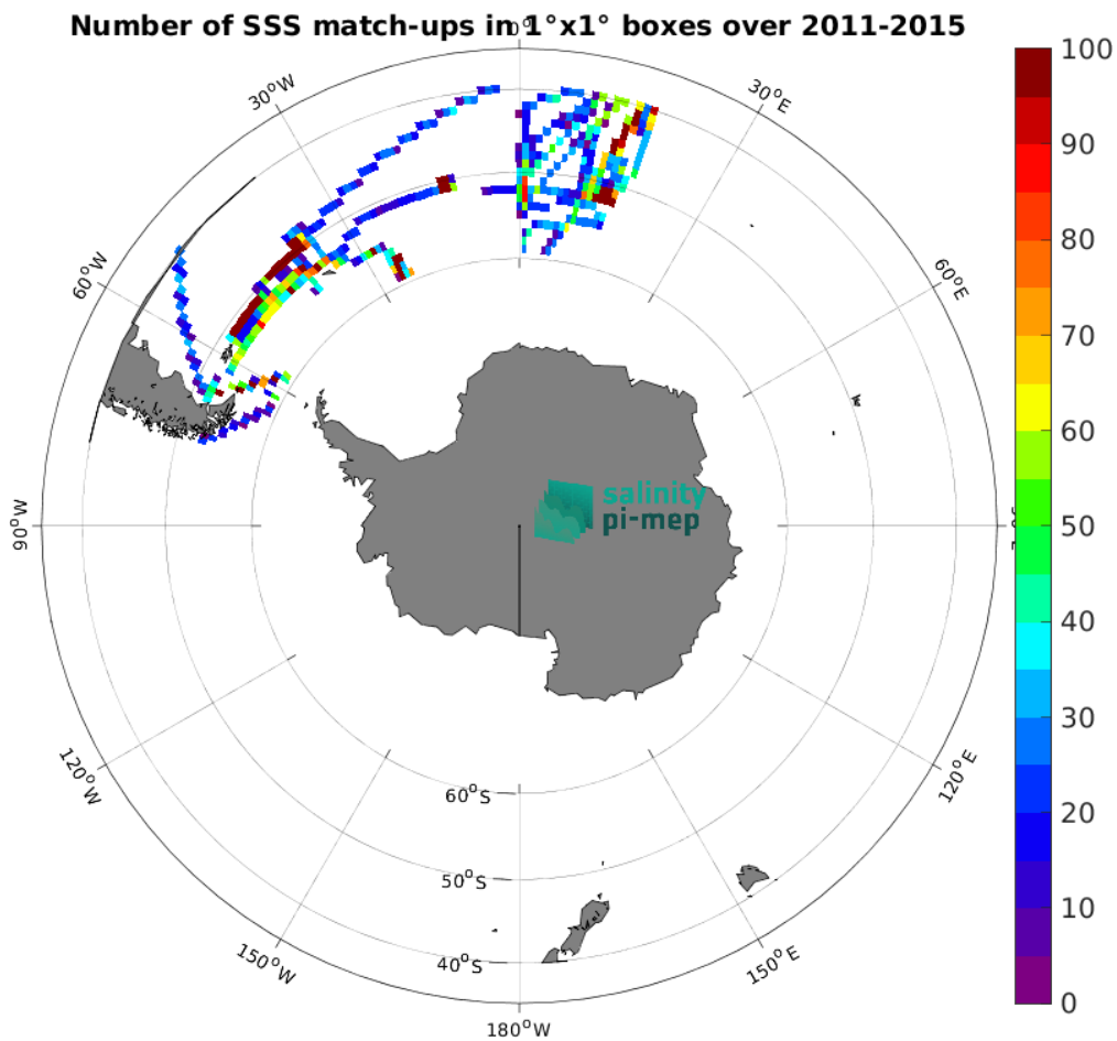
Figure 5: Number of SSS match-ups between TSG (Polarstern) SSS and the Aquarius SSS L3 OR v5 - 7-Day running - Rain mask (NASA-GSFC) SSS product for the Roaring Forties and Furious Fifties Pi-MEP region over 1^\circ \times 1^\circ boxes and for the full satellite product period.
