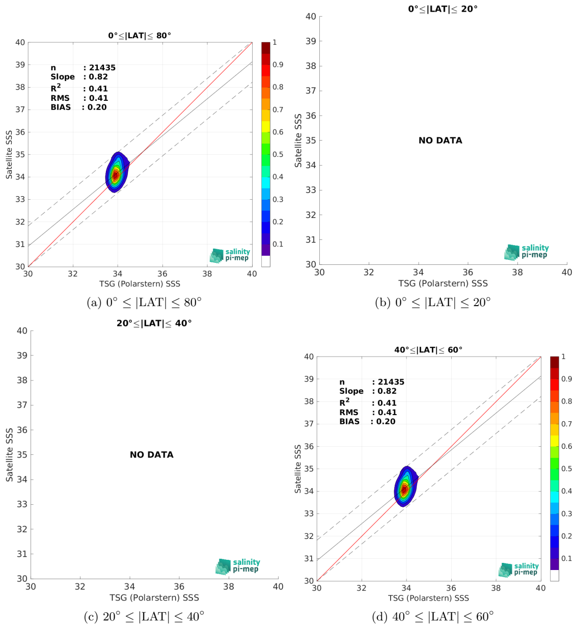
Figure 10: Contour maps of the concentration of Aquarius SSS L3 OR v5 - 7-Day running - Rain mask (NASA-GSFC) SSS (y-axis) versus TSG (Polarstern) SSS (x-axis) at match-up pairs for different latitude bands. For each plot, the red line shows x=y . The black thin and dashed lines indicate a linear fit through the data cloud and the \pm 95\% confidence levels, respectively. The number match-up pairs n , the slope and R^2 coefficient of the linear fit, the root mean square (RMS) and the mean bias between satellite and in situ data are indicated for each latitude band in each plots.
