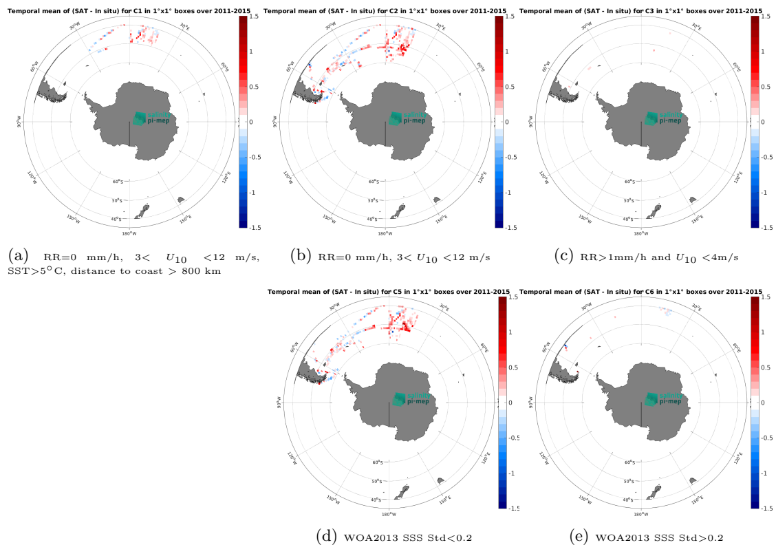
Figure 14: Temporal mean gridded over spatial boxes of size 1^\circ \times 1^\circ of \Delta SSS (Aquarius SSS L3 OR v5 - 7-Day running - Rain mask (NASA-GSFC) - TSG (Polarstern)) for 5 different subdatasets corresponding to:RR=0 mm/h, 3 < U_{10} < 12 m/s, SST > 5^\circ\text{C} , distance to coast > 800 km (a), RR=0 mm/h, 3 < U_{10} < 12 m/s (b), RR > 1 mm/h and U_{10} < 4 m/s (c), WOA2013 SSS Std < 0.2 (d), WOA2013 SSS Std > 0.2 (e).
