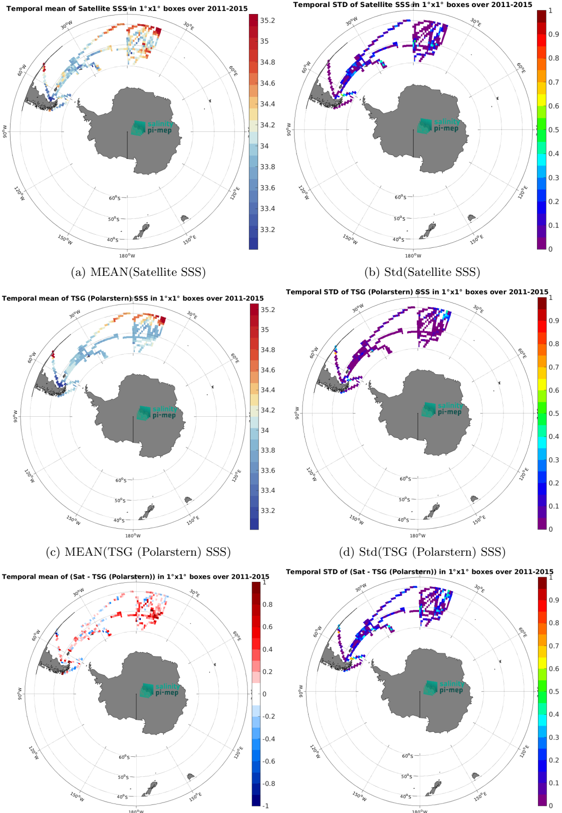
Figure 6: Temporal mean (left) and Std (right) of SSS from Aquarius SSS L3 OR v5 - 7-Day running - Rain mask (NASA-GSFC) (top), TSG (Polarstern) (middle), and of \Delta SSS (Satellite - TSG (Polarstern)). Only match-up pairs are used to generate these maps.
