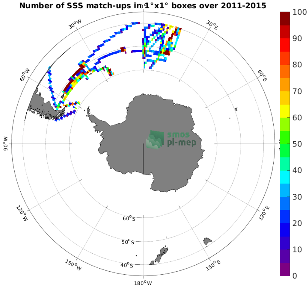
Figure 4: Number of SSS match-ups between TSG (Polarstern) SSS and the Aquarius SSS L3 OR v5 - 7-Day running - Rain mask (NASA-GSFC) SSS product for the Roaring Forties and Furious Fifties Pi-MEP region over 1^\circ \times 1^\circ boxes and for the full satellite product period.
